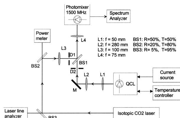
Fig. 1. Schematic of the optical setup for the beating experiment: BS1–BS3, beam splitters; L1–L3, lenses; D1, D2, beam waists; M, mirror.
