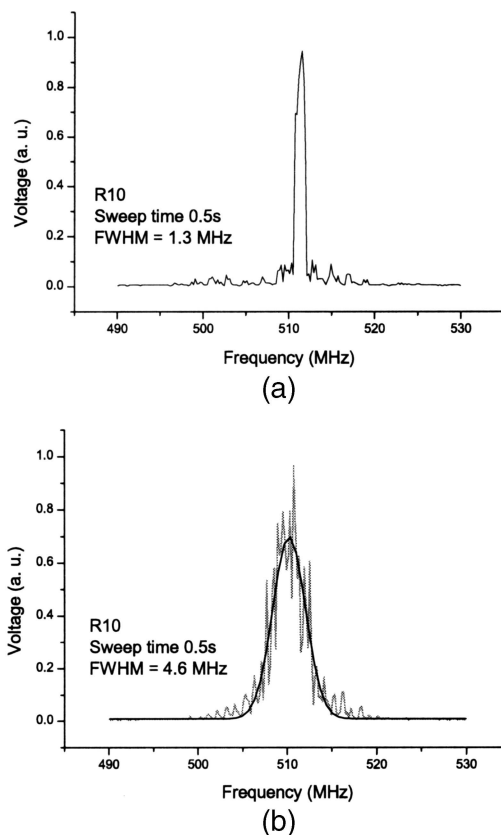
Fig. 2. Beat notes of the QCL operating at 0.47\text{ A} and 86.3\text{ K} and of the isotopic \text{C}^{18}\text{O}_2 laser lasing on the R10 line. (a) Low and (b) high linewidth limits observed under identical experimental conditions.
