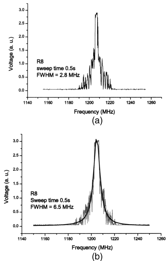
Fig. 3. Beat notes of the QCL operating at 0.85 A and 91 K and of the isotopic C^{18}O_2 laser lasing on the R8 line under the same experimental conditions as for Fig. 2.
