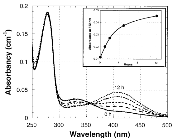
FIGURE 5: Release of \text{TNB}^- from DTNB-modified FBPAse mutant C174S. The labeled protein was incubated at 25 °C and spectra recorded at intervals. The spectra represented were recorded after 0, 1, 2, 5, 12 h incubation. The insert shows the time course of absorbency increase at 412 nm due to the release of \text{TNB}^- .
