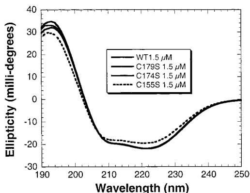
FIGURE 8: Circular dichroism spectra of 1.5 \mu\text{M} WT and mutant FBPsases in 10 mM potassium-phosphate, pH 6.0, were recorded in 0.1 cm path-length cuvettes.
