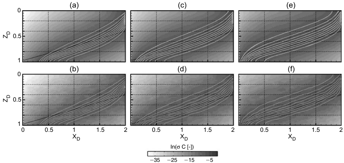
Fig. 5 Ergodicity test: upper row (a, c, e): 2D vertical cross-section ( y_D=0.5 ) of the ensemble average relative salt concentration [-] isolines (0.1–0.9) and the ensemble variance ( background greyscale map ) calculated on 100 3D simulations. Lower row (b, d, f): 2D view of the spatial average relative salt concentration [-] isolines (0.1–0.9) and the spatial variance calculated on a single 3D simulation. Greyscale maps represent the natural logarithm of the variance. The results are presented for l_x = l_y = 0.12 l_z = 0.04 and the three cases of \ln(K) variance (a – b \sigma_Y^2 = 1 , c – d \sigma_Y^2 = 2 , e – f \sigma_Y^2 = 3 )
