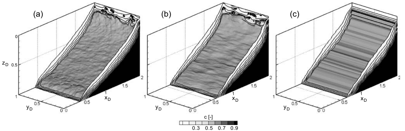
Fig. 8 3D view of the relative salt concentration [-] isolines (0.1–0.9); a for the isotropic case with l_x = l_y = l_z=0.04 , b for the case where l_x = l_z=0.04 and l_y=0.1 , c for the case with l_x = l_z=0.04 and l_y = +\infty . Note that c is equivalent to a 2D model. For the 3 cases, the \ln(K) variance is equal to 1
