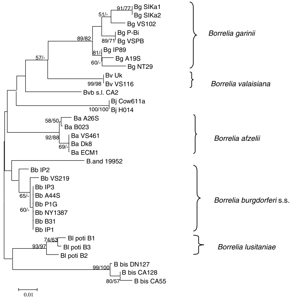
Fig. 1. Neighbour-joining tree of 1000 bootstrap pseudo-replicates with Kimura 2 parameters distances from recA sequences (162 bp) for 33 Borrelia strains. Numbers above branches indicate bootstrap support values higher than 50% for NJ/MP.
