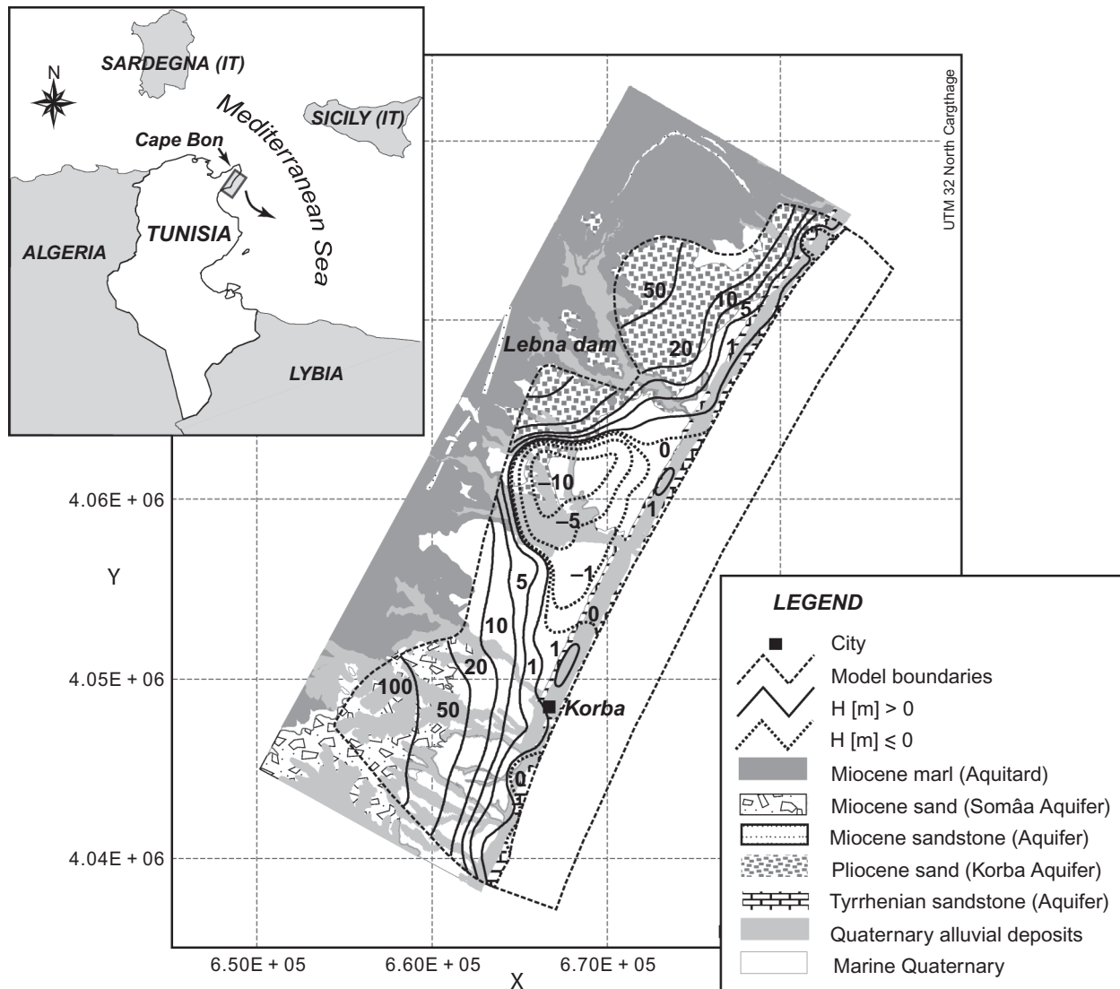
Fig. 1 Location map of the Korba aquifer and geological settings (squares are 10 \times 10 km). Hydraulic heads observed in August 2004 are also shown.
