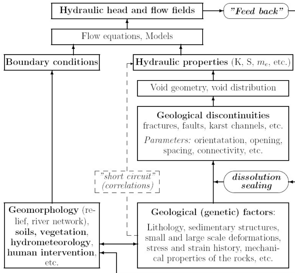
Figure 1: Schematic representation of the relations between groundwater flow field, hydraulic properties and geological factors in karst aquifers (after Kiraly 1975, modified).
