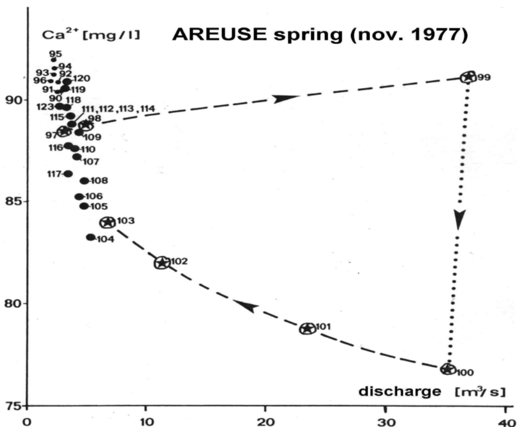
Figure 14: \text{Ca}^{2+} concentration versus discharge for the single peak shown in Fig. 13. Observe the dilution between samples 99 and 100 and the clustering of points located on the slow recession hydrograph (after Kiraly and Muller 1979).
