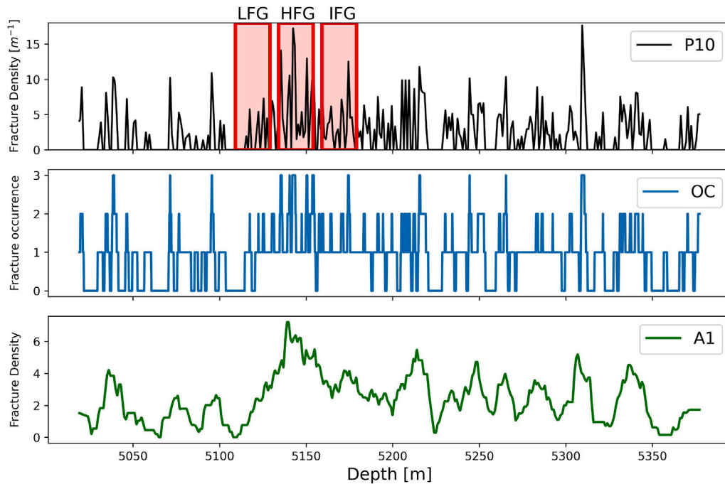
Fig. 3. Training data set from well-11 for gap filling: fracture density (P10), fracture occurrence (OC) and low frequency trend (A1). Highlighted gaps in red at the P10 track, where data set was excluded for cross-validation at the less fractured interval (LFG), higher fractured interval (HFG), and intermediate fracture interval (IFG).
