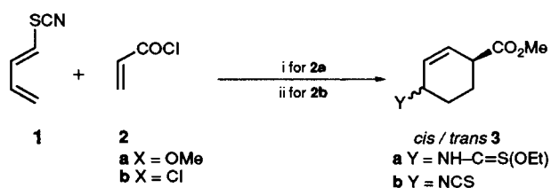
Scheme 1 Reagents and conditions: i, BHT, EtOH, 110 °C, 60%; ii, cat., toluene then MeOH, Et 3 N
