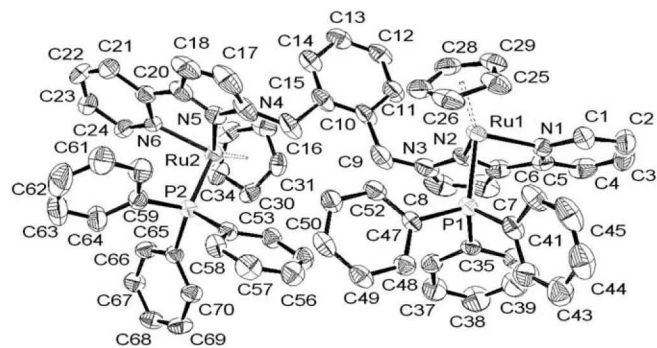
Fig. 3. Molecular structure of [(\eta^5\text{-C}_5\text{H}_5)_2\text{Ru}_2(\text{NN}\cap\text{NN})(\text{PPh}_3)_2](\text{PF}_6)_2 at 35% probability level. Hydrogen atoms, diethyl ether molecule and hexafluorophosphate anions have been omitted for clarity.
