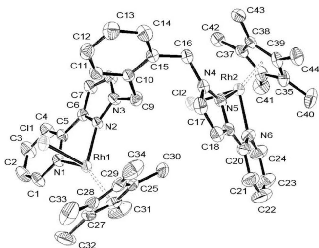
Fig. 2. Molecular structure of [(\eta^5\text{-C}_5\text{Me}_5)_2\text{Rh}_2(\text{NN}\cap\text{NN})\text{Cl}_2](\text{PF}_6)_2 at 35% probability level. Hydrogen atoms, water molecules and hexafluorophosphate anions have been omitted for clarity.
