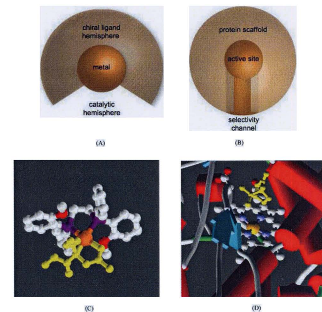
Fig. 1 Schematic representation of an enantioselective homogeneous catalyst (A) and of an enzyme (B); structure of Knowles's \{\text{Rh}(\text{DIPAMP})\}^+ bound to its substrate (yellow), emphasizing the limited space (hemisphere) occupied by the enantiopure ligand (CSD ref. code: VERYAS). Note the orientation of the phenyl groups bound to phosphorus: the o -anisyl presents its face while the phenyl group presents its edge (C); structure of cytochrome P450 cam with its substrate (camphor, yellow), emphasizing the “lock and key” complementarity between the enzyme and its substrate (pdb ref. code: 2CPP) (D).
