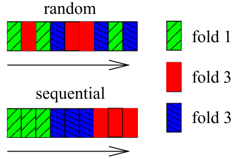
Fig. 1. Cross-validation illustration on a dataset with t = 9 records. We perform 3-fold cross-validation. Each fold is represented by a different colour. In random cross-validation, folds are assigned randomly to each record. In the sequential variant, folds are assigned sequentially.
