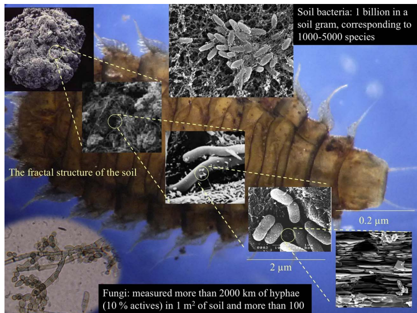
Fig. 19. The fractal nature of soil structure. Pictures at different scales were found online and were reassembled. In background the photograph of a Fannia fly larva found in a Moder in the Fontainebleau forest. The size of this small animal (3–4 mm) may be compared to one of the largest aggregates (1–2 mm) placed in the upper left corner. The figure illustrates the complexity of the soil world. The human mind is rather accustomed to apprehend objects at a “visible to naked eye” scale. The functional value of structures smaller than 1/10 mm is thus often overlooked. We breath, drink and eat a lot of bacteria, we are covered by billions of microorganisms but we never think to them unless we are ill. The same happens when we look at the soil. Making a hole, we move billions of microorganisms (Florenzano, 1972), but we do not think to them and generally classify the soil without considering this immense natural force (A. Zanella, A. Squartini).
