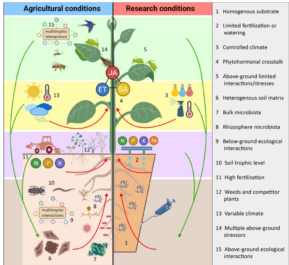
Figure 1. The context-dependency of ISR. Simplified representation of biotic and abiotic factors that can impact successful ISR activation under agricultural field conditions ( left ) and controlled research conditions ( right ). From bottom to top, red arrows indicate the progression of ISR activation from the onset at the root level to systemic transmission. Colored boxes indicate possible factors impacting activation of ISR at different stages of the process. Following the process from bottom to top: (brown) belowground triggering of ISR, (purple) impact of soil nutrient availability and plant nutritional status, (yellow) integration of systemic responses through crosstalk between signaling pathways activated by the beneficial microbes and abiotic environmental stressors, and (green) multiple above-ground stressors. Green arrows indicate cascading top-to-bottom effects that impact plant–microbe interactions belowground, and red arrows indicate bottom-up effects and environmental factors that potentially alter plant–microbe interactions and therefore ISR. Differences between the two environmental conditions ( left, right ) lead to variation in plant-beneficial microbe interactions and therefore differences in the potential to activate ISR, although microbial ISR activation under agricultural conditions is less explored. This image was made with © BioRender-biorender.com.
