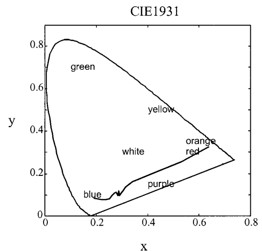
Fig. 12 Color trace of the double layer with pitches of 265 and 395 nm starting in the reddish orange (pitch, 395 nm) and ending in the purplish blue (pitch, 265 nm).
