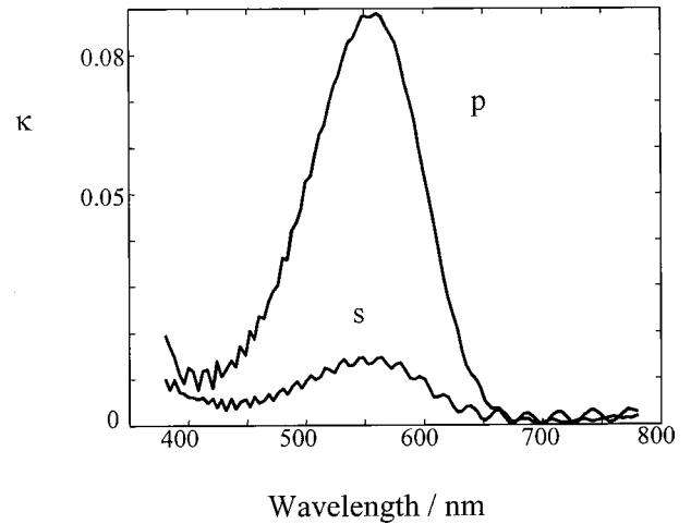
Fig. 7 Spectral absorption coefficient of an LC layer with 1 wt% D35. The two curves are related to the s and p polarizations.
