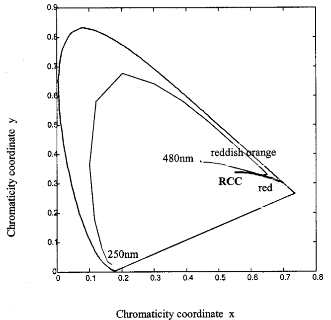
Fig. 1 Color coordinates in the chromaticity diagram CIE1931 for reflection spectra of a CLC with different pitches starting from 250 to 480 nm with an increment of 10 nm.
