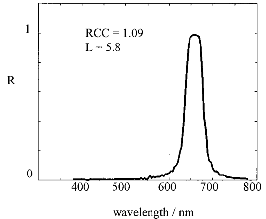
Fig. 11 Reflection spectrum generated by the index profile shown in Fig. 10. The pitch of the CLC is 400 nm.
