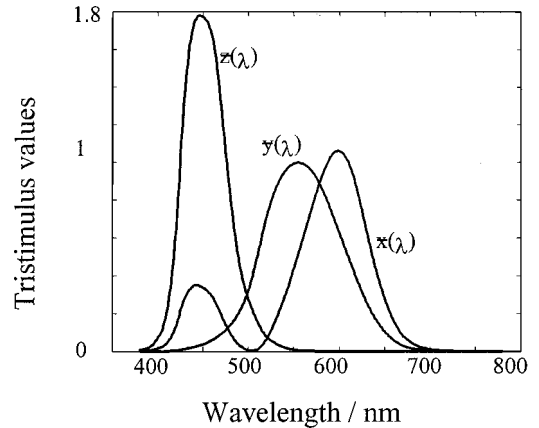
Fig. 4 Color-matching functions of CIE1931 standard colorimetric observer [ z(\lambda), y(\lambda), x(\lambda) ]. The y curve is also known as the photopic spectral eye sensitivity, which has its maximum at 555 nm.
