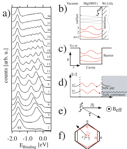
FIG. 1 (color online). (a) Quantum well states as seen by ultraviolet photoemission [modified VG Escalab MkII with a monochromatized hydrogen Ly_{\alpha} ( h\nu = 10.2 eV) photon source] in normal emission geometry at T = 300 K. States above the surface state energy at -1.7 eV are QWS. The film thickness for the spectra is given in units of unit cells ( 5.21 Å), comprising two atomic layers. (b) Experimental cavity with surface and interface boundary and three cavity modes. An off-normal quantum well state, characterized by a wave vector component parallel to the surface, k_{\parallel} , indicating a sideways displacement. (c) Ideal cavity with infinitely high walls. (d) Difference between a confined quantum well state and a leaky quantum well resonance with a corresponding change in wavelength. (e) Vectorial representation of the effective in-plane magnetic field, B_{\text{eff}} , at the Rashba interface. (f) Brillouin zones with high symmetry points for the epitaxial relationship between the sixfold symmetric ( C_6 ) Mg(0001) thin film and the twofold symmetric ( C_2 ) W(110) substrate.
