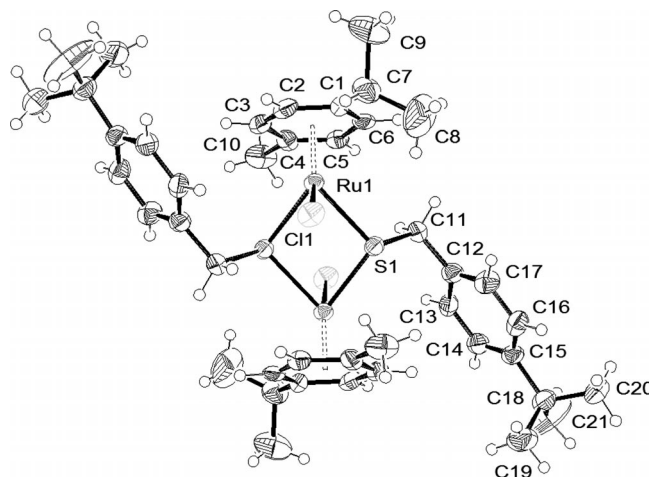
Figure 1. Molecular structure of 3 at 50% probability level ellipsoids. Selected bond lengths [Å] and angles [°]: Ru1–S1 2.384(2), Ru1–S1 i 2.395(3), Ru1–Cl1 2.424(2), Ru1–Ru1 i 3.674(2); S1–Ru1–S1 i 79.51(9), S1–Ru1–Cl1 81.16(8), S1 i –Ru1–Cl1 90.19(9), Ru1–S1–Ru1 i 100.49(9). Symmetry operator: i 1 – x , – y , 1 – z .
