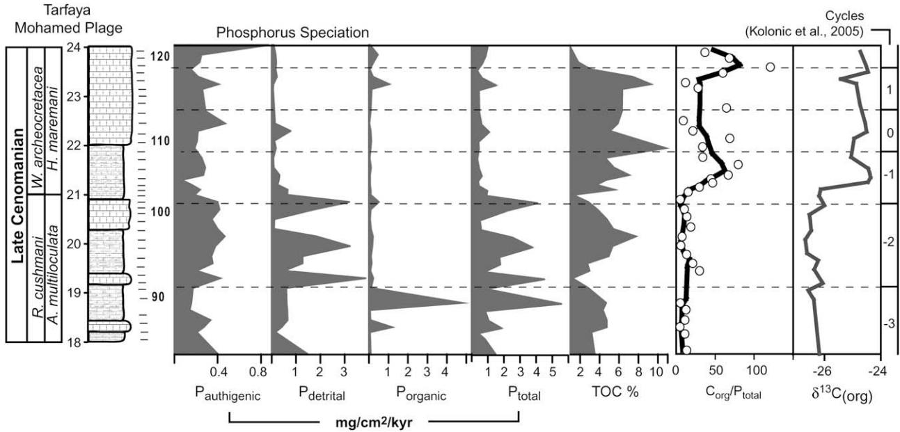
Fig. 8. Results from a sequential extraction of phosphorus (including P_{\text{authigenic}} apatite, P_{\text{detrital}} and P_{\text{organic}} ). P_{\text{reactive}} is taken as an addition of these phases. C_{\text{org}}/P_{\text{reactive}} (Redfield) ratios are also calculated and included alongside TOC and \delta^{13}\text{C}_{\text{(org)}} data.
