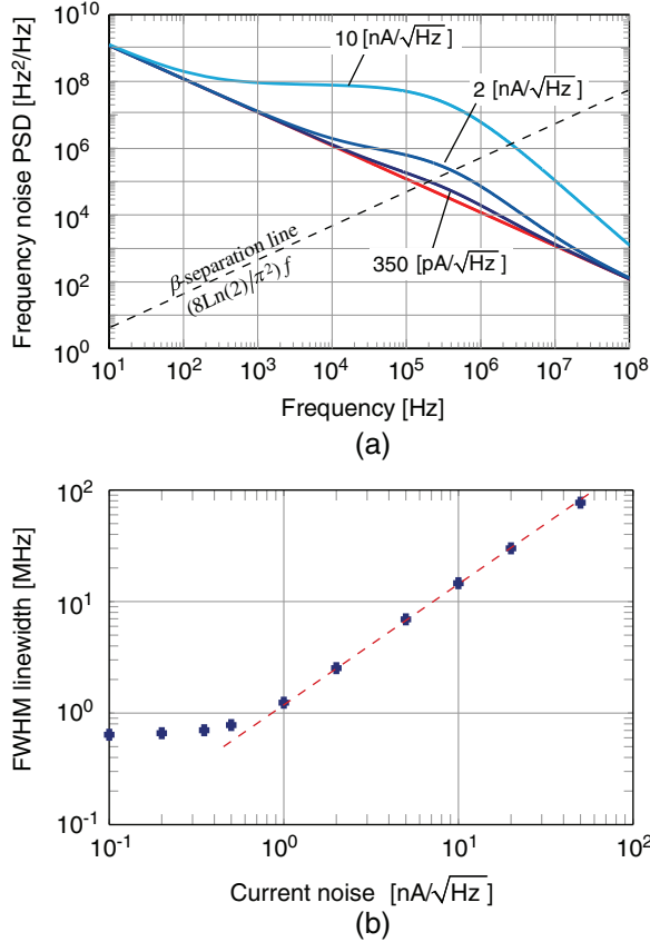
Figure 12.4 (a) Simulation of the laser frequency noise induced by drivers with different current noise densities. (b) Calculated laser linewidth (FWHM) as a function of the driver current noise density (white current noise is considered). The dashed line represents the linear broadening rate [ \sim 1.6 \text{ MHz}/(\text{nA}/\sqrt{\text{Hz}}) ] of the laser linewidth as a function of the current noise (reprinted from Ref. 24).
