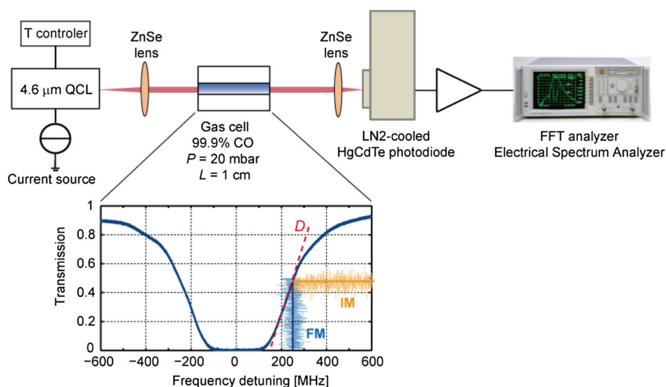
Figure 12.2 Scheme of the experimental setup used to measure the frequency noise of a QCL at 4.6\ \mu\text{m} . The R(14) CO absorption profile measured in the gas cell is shown in the lower part of the figure. The linear side of the absorption profile is used as a frequency discriminator to convert frequency noise (FM) into intensity noise (IM). The discriminator slope D is indicated by the dashed line.
