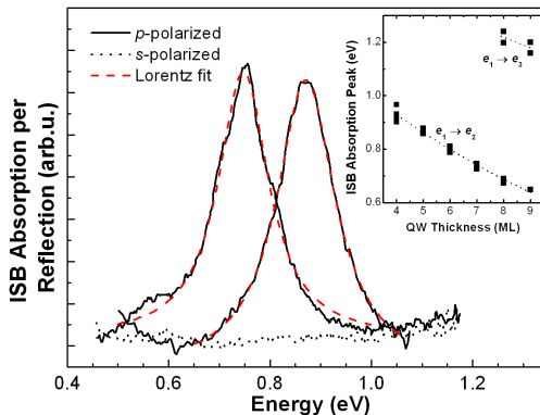
Fig. 2. Room-temperature ISB absorption spectra of AlN/GaN MQW structures for p -polarized and s -polarized light. The QW thicknesses are equal to 5 ML and 7 ML. Dashed lines present Lorentzian fits of the spectra. Inset: Variation of the e_1 \rightarrow e_2 and e_1 \rightarrow e_3 ISB absorption peaks as a function of the QW width, for samples doped in the QWs at 5 \times 10^{19} \text{ cm}^{-3} .
