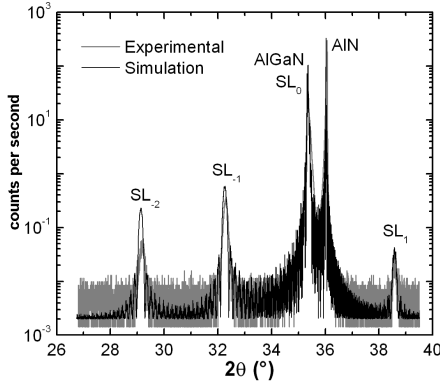
Fig. 3. HRXRD \theta - 2\theta scan of the (0002) reflection of a QWIP structure. Superlattice (SL) satellite peaks up to the second order are clearly visible, whereas the SL zero-order reflection peak ( SL_0 ) overlaps with the \text{Al}_{0.65}\text{Ga}_{0.35}\text{N} reflection. An average period of 2.93 nm is obtained from the inter-satellite distance. The simulation was performed using the program X’Pert Epitaxy 40 from Phillips Analytical, assuming that the structure is fully strained on the AlN buffer.
