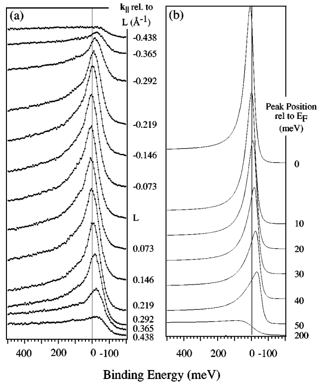
FIG. 2. (a) Angle resolved photoemission (ARPES) spectra in the (\Gamma ALM) plane vs the binding energy, carried out with He-I \alpha radiation at room temperature. Only spectra near the L point are displayed (see text). (b) Simulation of the ARPES spectra from (a) for varying initial state energy positions (cf. text).
