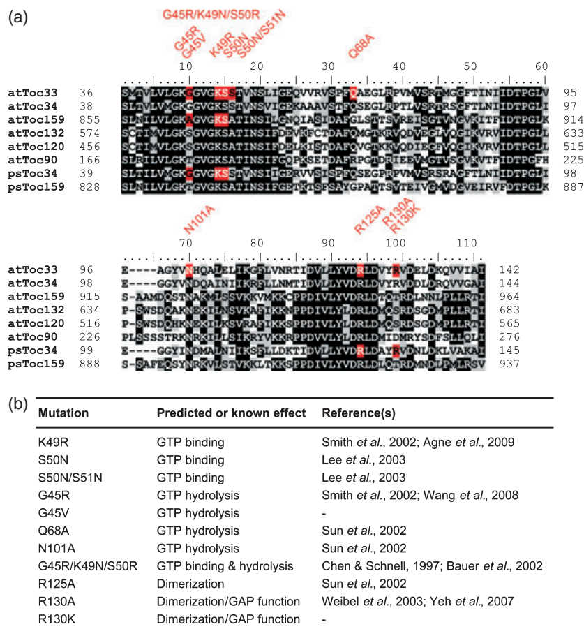
Figure 1. Details of the atToc33 mutations used in this study.
