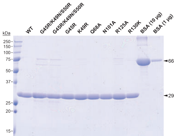
Figure 2. Recombinant atToc33 proteins for in vitro studies. Recombinant wild-type (WT) and mutant (G45R/K49N/S50R, G45R, K49R, Q68A, N101A, R125A and R130K) atToc33 proteins lacking the C-terminal transmembrane domain were resolved by SDS-PAGE and stained with Coomassie Blue. Each lane contains \sim 5 \mu\text{g} of recombinant protein. To confirm sample concentrations, 10- \mu\text{g} and 1- \mu\text{g} aliquots of BSA were also loaded. Molecular weight standards are indicated in kDa.
