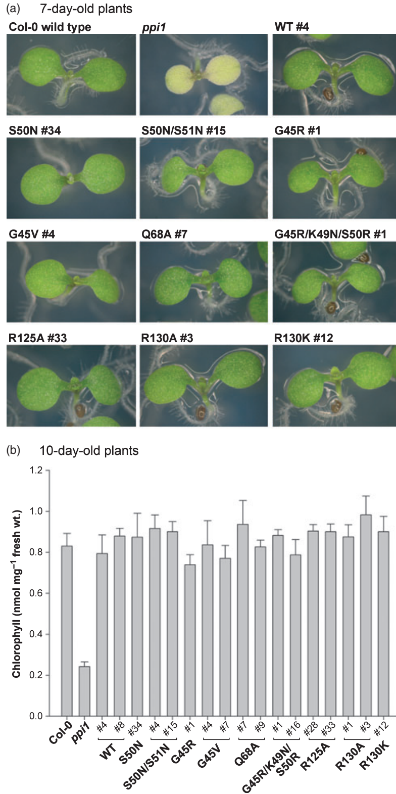
Figure 6. Basic characterization of transgenic ppi1 plants expressing atToc33 mutant constructs.
