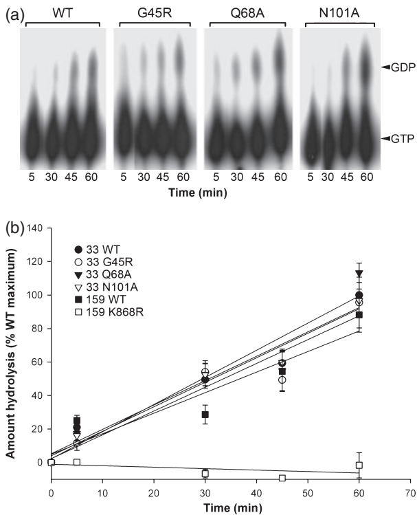
Figure 4. In vitro analyses of nucleotide hydrolysis by the atToc33 mutants. (a) Recombinant atToc33 proteins were incubated with [ \alpha - ^{32} P]GTP for 5, 30, 45 and 60 min. Samples were then separated by TLC and visualized by autoradiography. The lower band in each case represents non-hydrolysed GTP, and the upper band represents GDP. (b) Radioactivity associated with the bands in panel (a), and with those from several similar experiments, was quantified and used to calculate the degree of GTP hydrolysis at each time point. One of the non-binding atToc33 mutants, K49R, was analysed as a negative control; the K49R mutant was selected as it was more efficiently purified than any of the other binding-defective mutants (Figure 2). Trace levels of GTPase activity detected using the K49R preparation (not shown) were attributed to small quantities of contaminating protein, and so the data for this mutant were used to normalize those for the putative hydrolytic mutants. The atToc159 proteins were expressed and purified as GST fusions, and so the corresponding data were normalized using a control GST preparation. The data presented are means ( \pm SE) derived from five or six independent experiments, and all are expressed as a percentage of the wild-type atToc33 60-min value.
