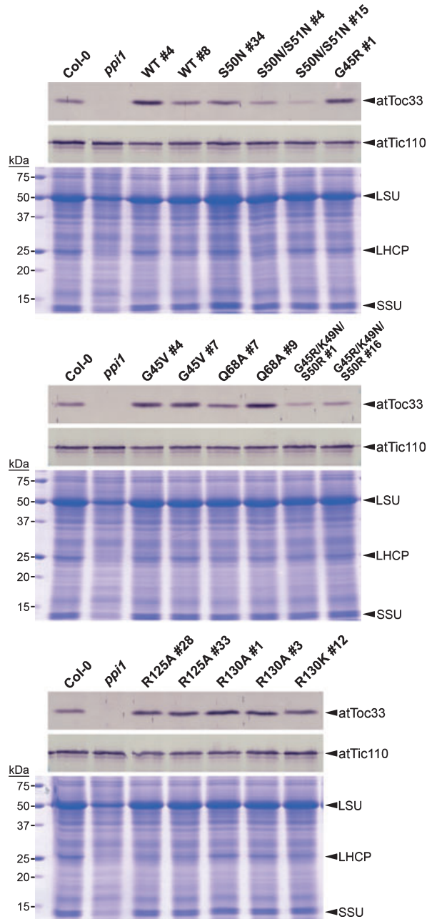
Figure 7. Immunoblots showing the expression of atToc33 proteins in the transgenic ppi1 plants.
