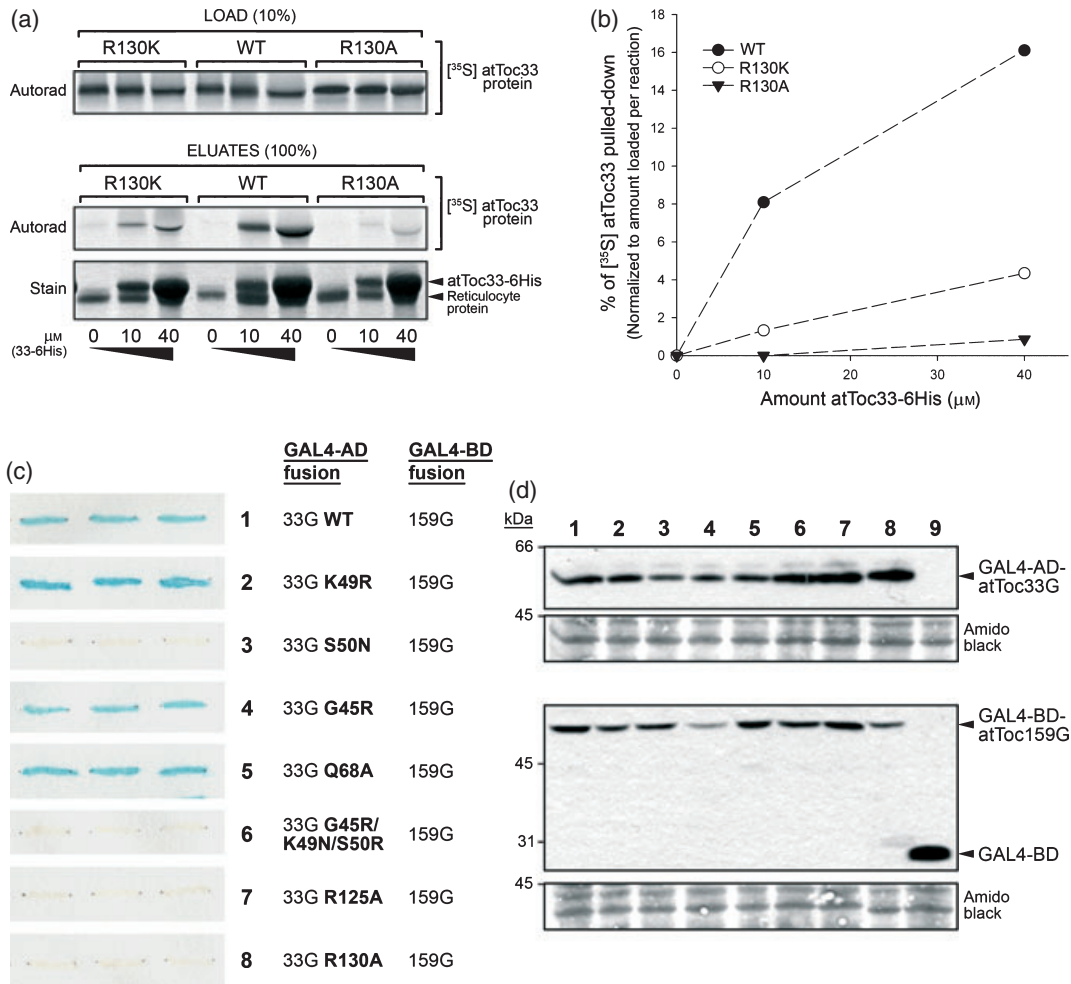
Figure 5. Homodimerization and heterodimerization of selected atToc33 mutants.
