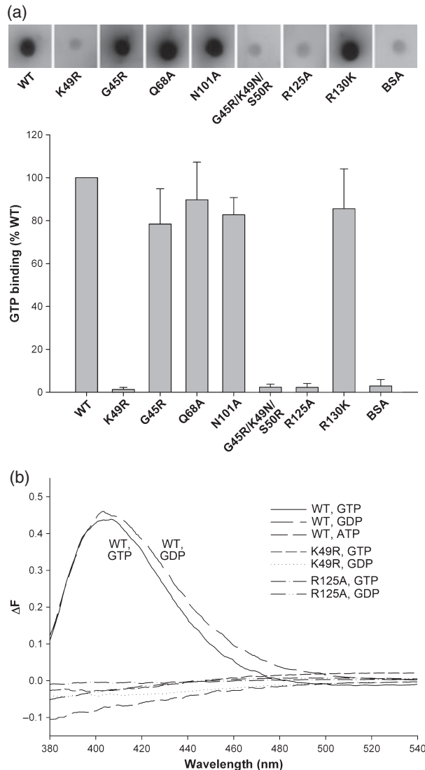
Figure 3. In vitro analyses of nucleotide binding to the atToc33 mutants.
