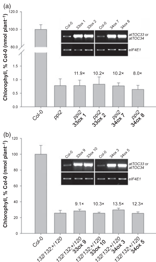
Figure 10. Overexpression of atToc33 and atToc34 in ppi2 and toc132 toc120 mutant plants.
