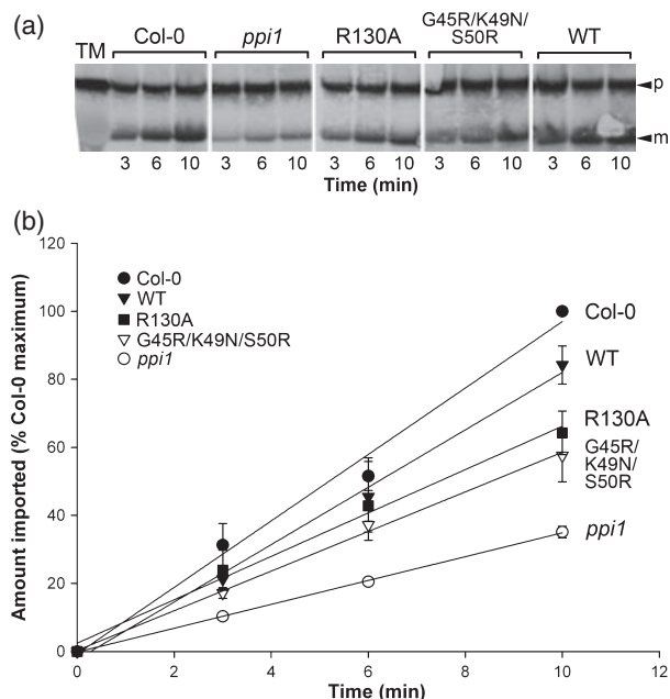
Figure 9. Analysis of the efficiency of pre-protein import into chloroplasts isolated from ppi1 plants expressing mutant atToc33 proteins.
