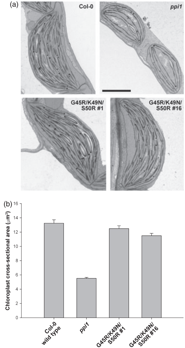
Figure 8. Ultrastructural analysis of chloroplasts in ppi1 plants expressing the G45R/K49N/S50R construct.
