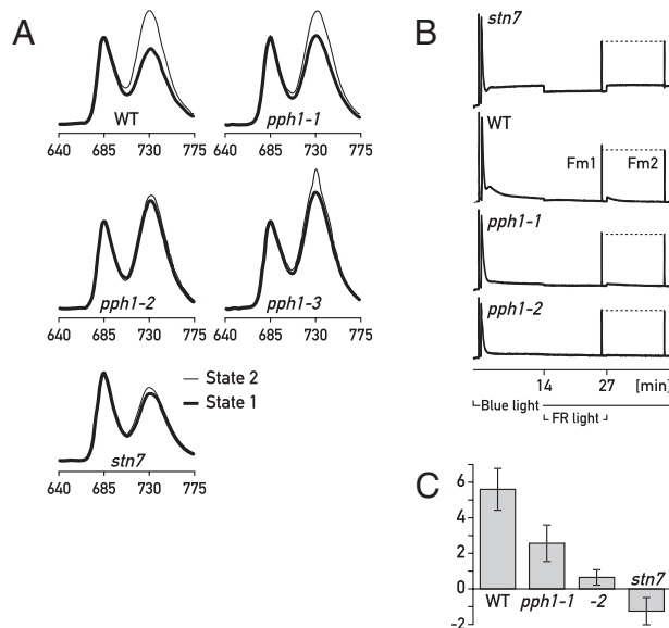
Fig. 4. Analysis of state transitions. (A) Chlorophyll fluorescence emission spectra at low temperature. Rosette leaves from Col0 wild type, three pph1 alleles, and stn7 grown in short days under white light were treated for 30 min under far-red (state 1 conditions) or blue light (state 2 conditions). Crude extracts were frozen in liquid nitrogen, and fluorescence emission spectra were obtained with excitation at 480 nm. Curves were normalized for the PSII peak at 685 nm (average of four measurements). Fluorescence emission peak from PSI was at \approx 732 nm. (B) Chlorophyll fluorescence analysis at room temperature. State transitions were measured with a pulse amplitude-modulated fluorimeter to monitor changes in the light-harvesting antenna associated with PSII. A dark-adapted leaf was exposed to blue light to induce state 2, then with additional far-red light to promote a transition to state 1, and was induced to return to state 2 after the far-red light was switched off. State transitions were estimated as the difference in maximal fluorescence in state 1 ( F_{m1} ) and in state 2 ( F_{m2} ), which was abolished in stn7 , strongly reduced in pph1-1 , and barely detectable in pph1-2 . State transitions are also denoted by small changes in fluorescence when the lights are switched. These reflect changes in the redox state of the plastoquinone pool. In stn7 , where the LHCII antenna stayed associated with PSII in blue light and the plastoquinone pool remained reduced, the decrease in fluorescence when the far-red light was turned on was more pronounced than in the wild type, where the state transition led to a gradual oxidation of the plastoquinone pool in blue light. As could be expected for a phosphatase mutant that favors state 2, only minor fluorescence changes were observed in pph1-1 and pph1-2 because the plastoquinone pool stayed predominantly oxidized. (C) Quantification of state transitions measured as in B: qT = (F_{m1} - F_{m2})/F_{m1} \times 100 (average of four different leaves, mean \pm SD).
