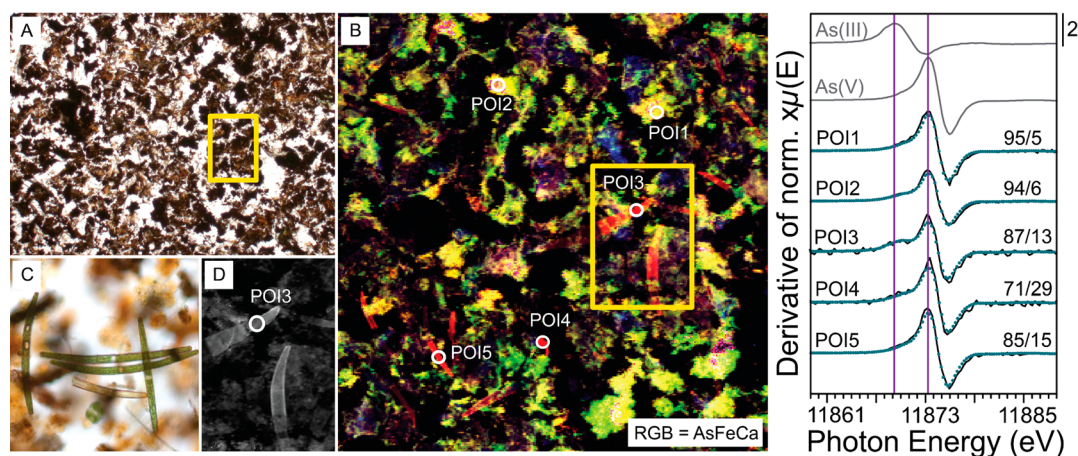
Figure 4. (A, C) Light microscopy and (B, D) \mu -XRF maps collected at 13 keV for floc sample W3. Image sizes are (H \times V) (A) 4 \times 3 \text{ mm}^2 , (B) 1.5 \times 1.5 \text{ mm}^2 , (C) 0.5 \times 0.5 \text{ mm}^2 , and (D) 0.3 \times 0.5 \text{ mm}^2 . Map (B) shows the distributions of As, Fe, and Ca, whereas the gray scale map (D) shows solely the distribution of As (white corresponds to high As concentrations). The yellow insets in (A) and (B) correlate with map (D). The right panel shows the first derivatives of As K-edge XANES spectra collected at selected points of interest (POIs) indicated in map (B). Their corresponding LCFs using arsenite/arsenate-adsorbed ferrihydrite as fit references are shown as dotted lines (fit range: -20 to 30 \text{ eV} ( E-E_0 ), initial fit sums: 100 \pm 10\% , normalized sum of squared residuals: 0.09 – 0.54\% ). The LCF results are reported as As(V)/As(III) ratios. Additional \mu -XRF maps are shown in SI Figures S12 and S13.
