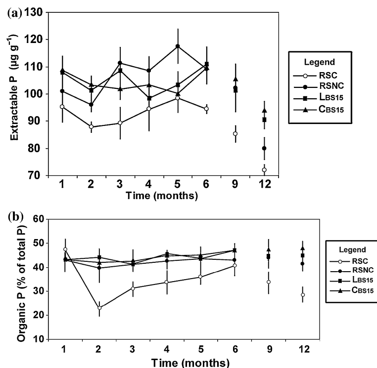
Figure 3. Soil bicarbonate extractable P (a) on a dry weight soil basis, and soil organic P (b) at different times from beginning of the experiment. L BS15 : soil from side arms of microcosms planted with lupin, 10–15 cm from roots; C BS15 : soil from side arms of microcosms without lupin; RSC: rhizosphere soil from cluster roots; RSNC: rhizosphere soil from non-cluster roots. Means and standard errors of means of three replicates are shown.
