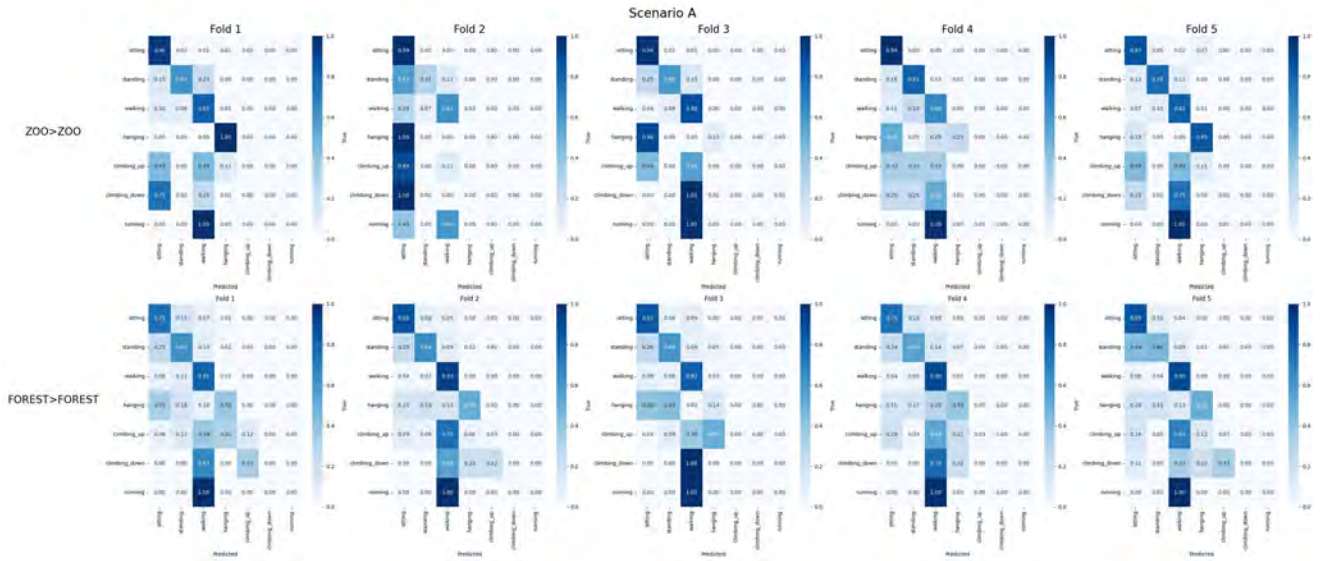
Figure 8. Confusion matrices for each fold in cross-validation: Scenario A - Within-dataset
