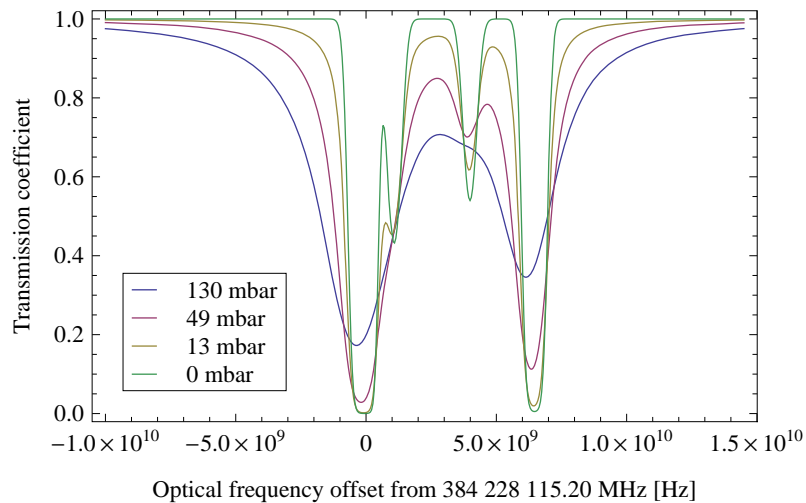
FIGURE 1.10: Transmission spectra computed for identical conditions except the buffer gas pressure.
