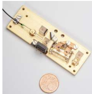
FIGURE 2.7: SQUATOS functional demonstrator. Dimensions of the base plate are 71 \text{ mm} \times 24 \text{ mm} [10].
