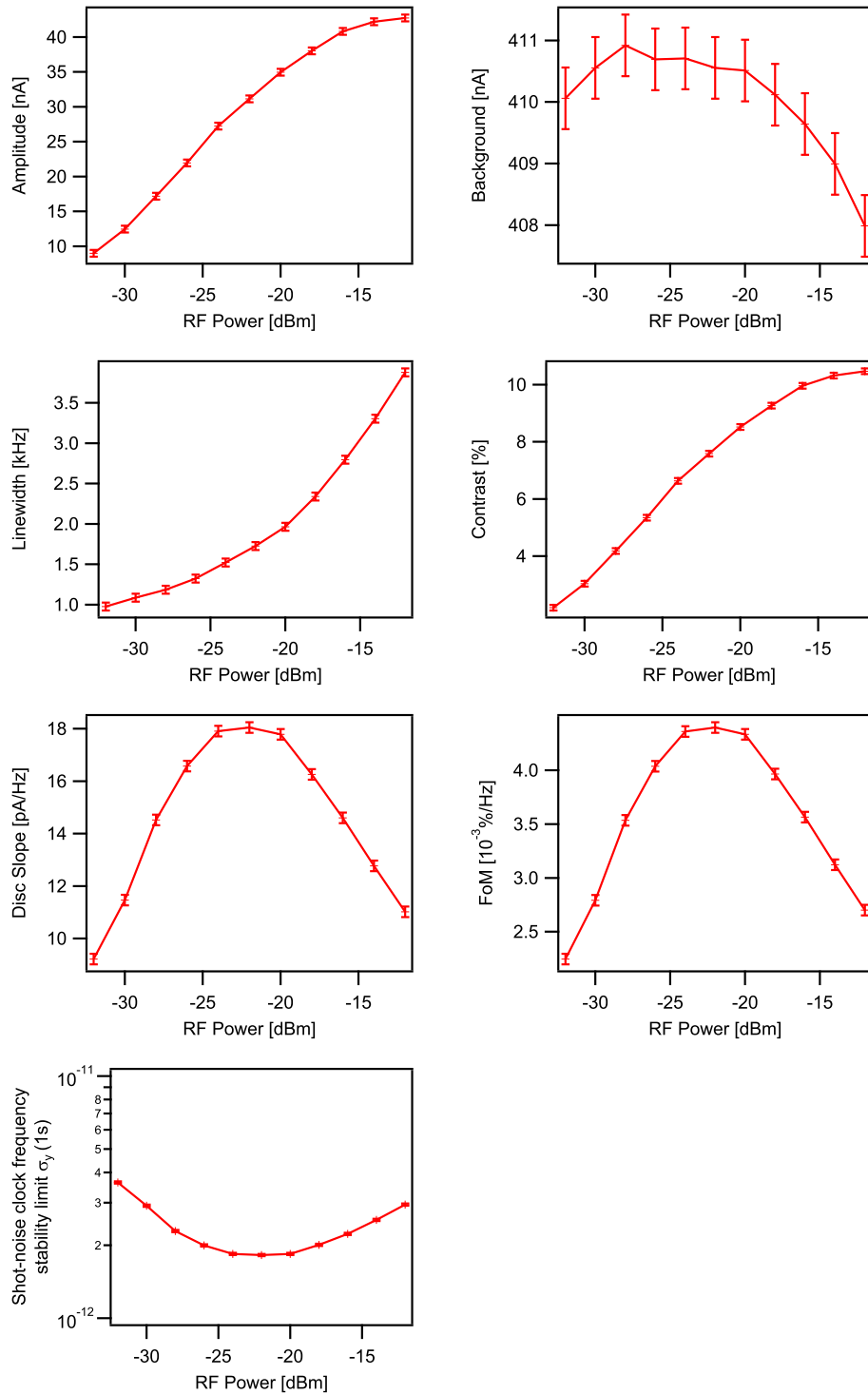
FIGURE 6.4: Clock signal parameters as a function of microwave power. The light intensity is fixed at 1 \mu\text{W}/\text{mm}^2 . Contrast, Discriminator slope, figure of merit (FoM) and Shot Noise limit are calculated from the measured Amplitude, Background level and Linewidth.
