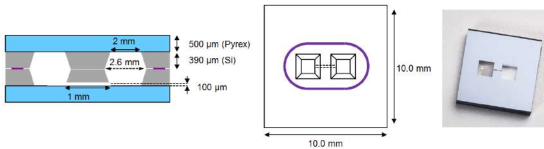
FIGURE 3.9: Design of the micro-fabricated coated cell. Courtesy: R. Straessle.
