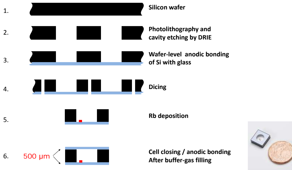
(A) 2D cell fabrication process flow [168].
