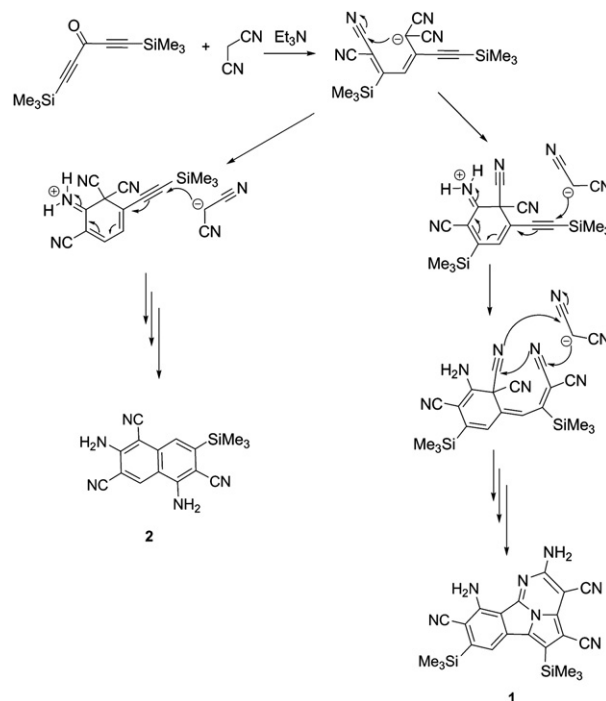
Scheme 2. Most plausible mechanisms for the formation of 1–2 .
