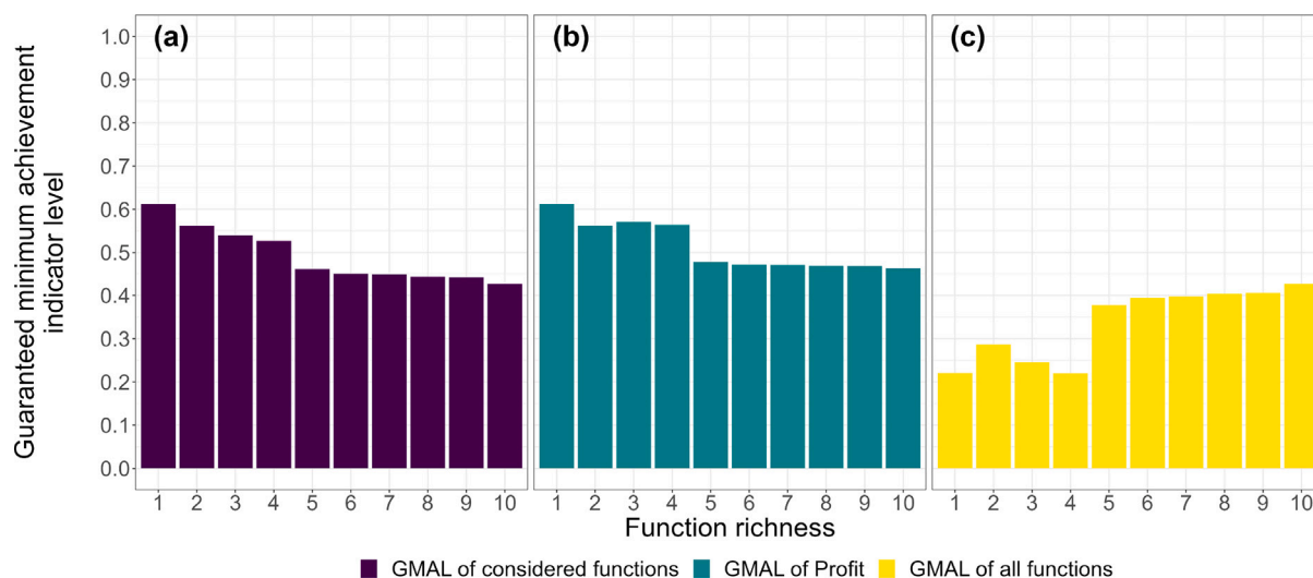
Fig. 3. The guaranteed minimum achievement indicator level (GMA) from three perspectives. (a) shows the GMA for each indicator set used to optimize portfolios with increasing function richness (robust performance of the considered functions) (Fig. 2). For example, all uncertainty scenarios of all five indicators, i.e., function richness of 5, achieve at least a performance of 0.46. (b) shows the GMA of solely the indicator Profit (robust performance of currently important function). The minimum achievement level of a function richness of 1 is thus equal in (a) and (b). (c) shows the GMA over all ten indicators for each portfolio with increasing function richness (robust multifunctionality). The GMA of function richness 10 is thus equal in (a) and (c).
