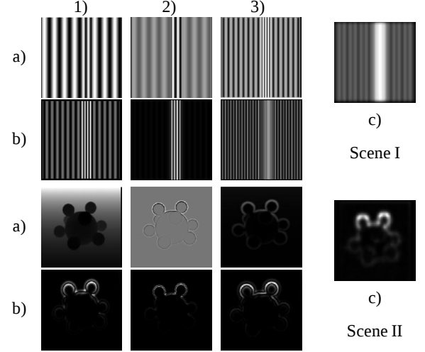
Figure 3. Computing the saliency map using 1) depth , 2) mean curvature and 3) depth gradient norm . a) feature maps, b) corresponding conspicuity maps and c) saliency map.
