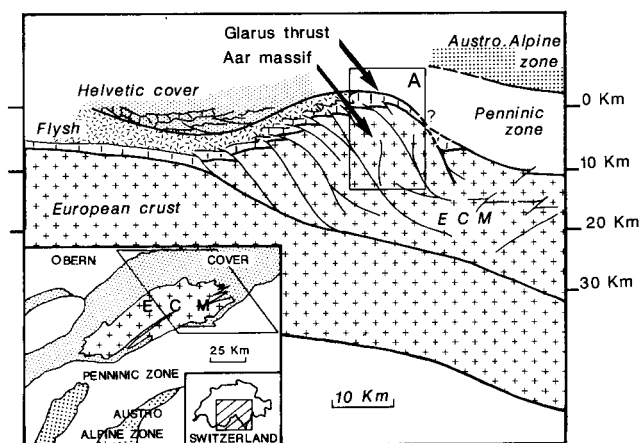
Fig. 1. General cross-section of the northern part of the Alps in eastern Switzerland before late Tertiary uplift (modified after Pfiffner et al. 1990a). E.C.M.: External Crystalline Massifs (Aar, Tavetsch and Gotthard). Black frame A is shown in Fig. 2.
