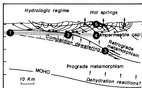
Fig. 7. Sketch of potential fluid sources and fluid regimes at the crustal scale. A present-day cross-section of the eastern Swiss Alps (compare with Fig. 1) is used to discuss the relative position of the Aar Massif in space and time during its tectonic evolution from late Eocene (1) to its present situation (5) (see text for explanation).
