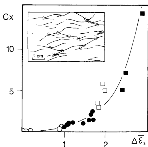
Fig. 4. Degree of shear band interconnection for variously deformed samples from the Grimsel granodiorite ( Cx = number of intersections per \text{cm}^2 ) vs relative finite strain intensity \Delta \bar{\epsilon}_s . The window shows an example of intersecting shear bands (open circles) in a sample of Grimsel granodiorite orthogneiss. Open circles: isotropic granodiorite; black circles: orthogneiss; white squares: mylonites; black squares: ultramylonites.
