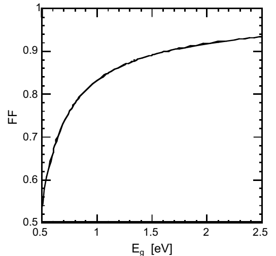
Fig. 3. Upper limit for the fill factor FF as a function of the energy gap E_g of the solar cell material based on an empirical minimum value (according to Green) for the reverse saturation current of the diode (Eq. (1)) and on above Eq. (3).
