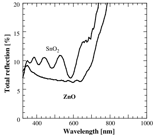
Fig. 8. Total reflection curves of glass/TCO/cell system, using either SnO 2 or ZnO as TCO layer.
