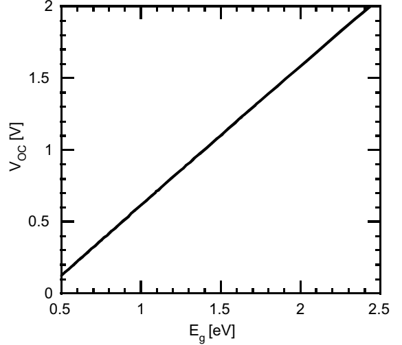
Fig. 2. Semi-empirical upper limit for the open-circuit voltage V_{oc} , as a function of the energy gap E_g of the solar cell material, based on Eqs. (1) and (2), hereunder.
