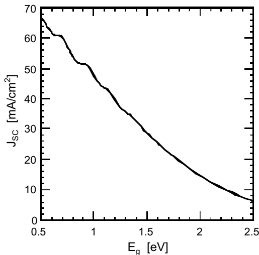
Fig. 1. Upper limit of the short-circuit current density J_{sc} as a function of the energy gap E_g of the solar cell material, under AM 1.5 illumination.
