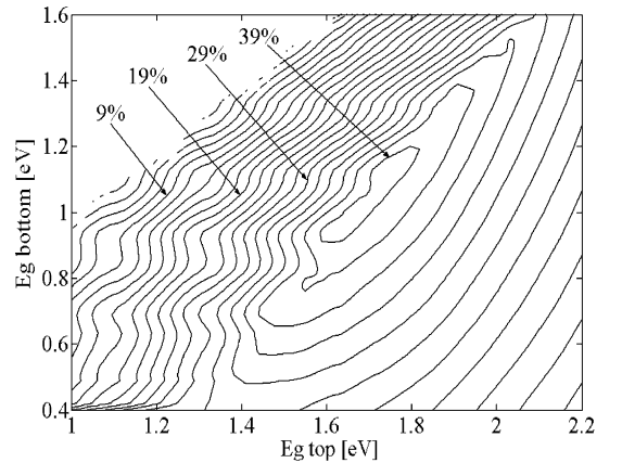
Fig. 5. Semi-empirical upper limit of the efficiency \eta as a function of the energy gap E_g of the bottom and top cells of a tandem solar cell based on an empirical minimum value (according to Green) for the reverse saturation current of the diode.
