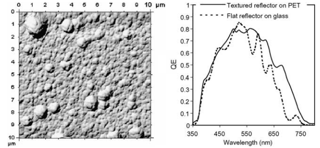
Fig. 9. AFM image of a performing randomly textured back reflector deposited on PET fabricated by \text{O}_2 -plasma; spectral response curve in the degraded state of a nip-type a-Si:H cell deposited thereon, as compared to an identical cell on a flat mirror-like back reflector on glass.
