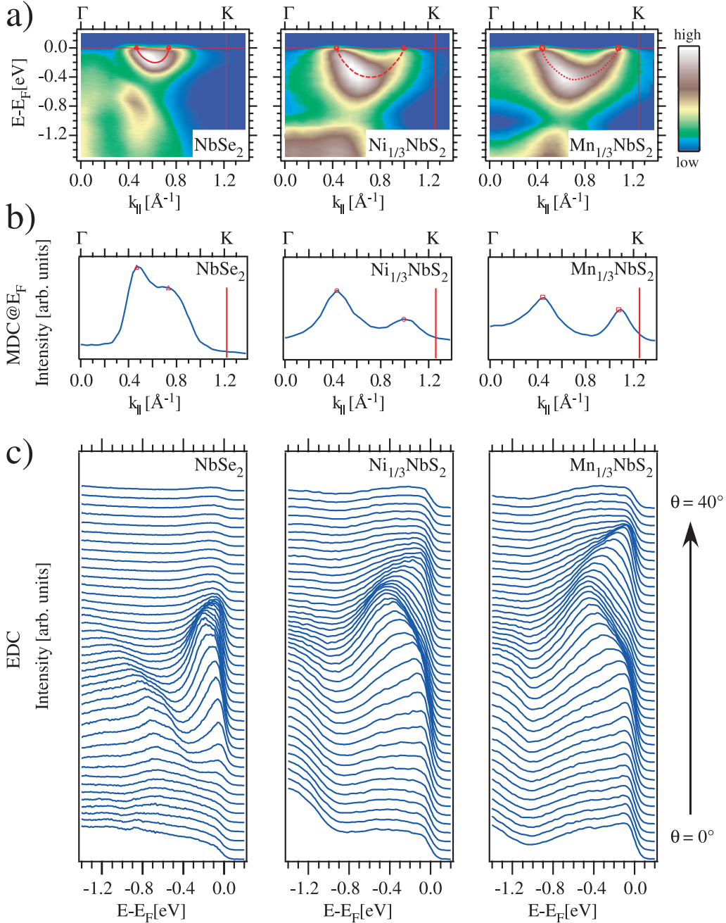
Fig. 2. (a) Comparison between ARPES dispersion maps along the \Gamma(A) - K(H) direction of NbSe 2 , Ni 1/3 NbS 2 and Mn 1/3 NbS 2 measured at room temperature. (b) MDCs extracted at the Fermi energy E_F as well as (c) EDCs stacked as a function of emission angles \theta are also shown. The red horizontal line marks the Fermi energy E_F , the red vertical line the position of the K(H) point. To guide the eye, the dispersion of the Nb 4d band is outlined by red curves. The Fermi vectors obtained from the MDCs are marked by red symbols.
