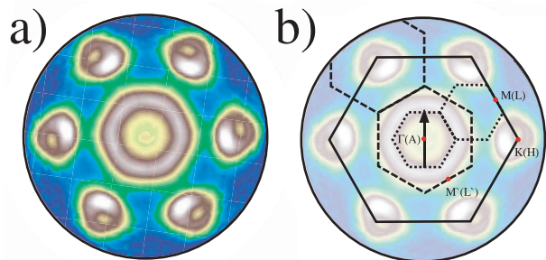
Fig. 1. (a) Fermi surface map of Mn_{1/3}NbS_2 at room temperature. The corresponding color scale is given in Figure 2a. (b) A sketch of the Brillouin zone of the host compound (full line) and of the \sqrt{3} \times \sqrt{3} (dashed line) and 3 \times 3 (dotted line) supercells with high symmetry points. High symmetry points in parenthesis are located on the top face of the hexagonal bulk Brillouin zone. The nesting vector corresponding approximately to the 3 \times 3 superlattice is also indicated.
