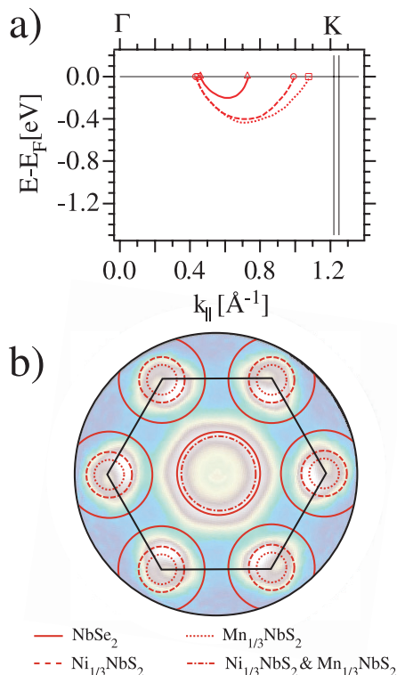
Fig. 3. Comparison between the Nb 4d band filling of \text{NbSe}_2 , \text{Mn}_{1/3}\text{NbS}_2 and \text{Ni}_{1/3}\text{NbS}_2 . (a) Summary of the dispersion maps from Figure 1a. Note the two positions of the K point due to the variation in lattice constant during intercalation. (b) Sketch of the effect of doping on the Fermi surface.
