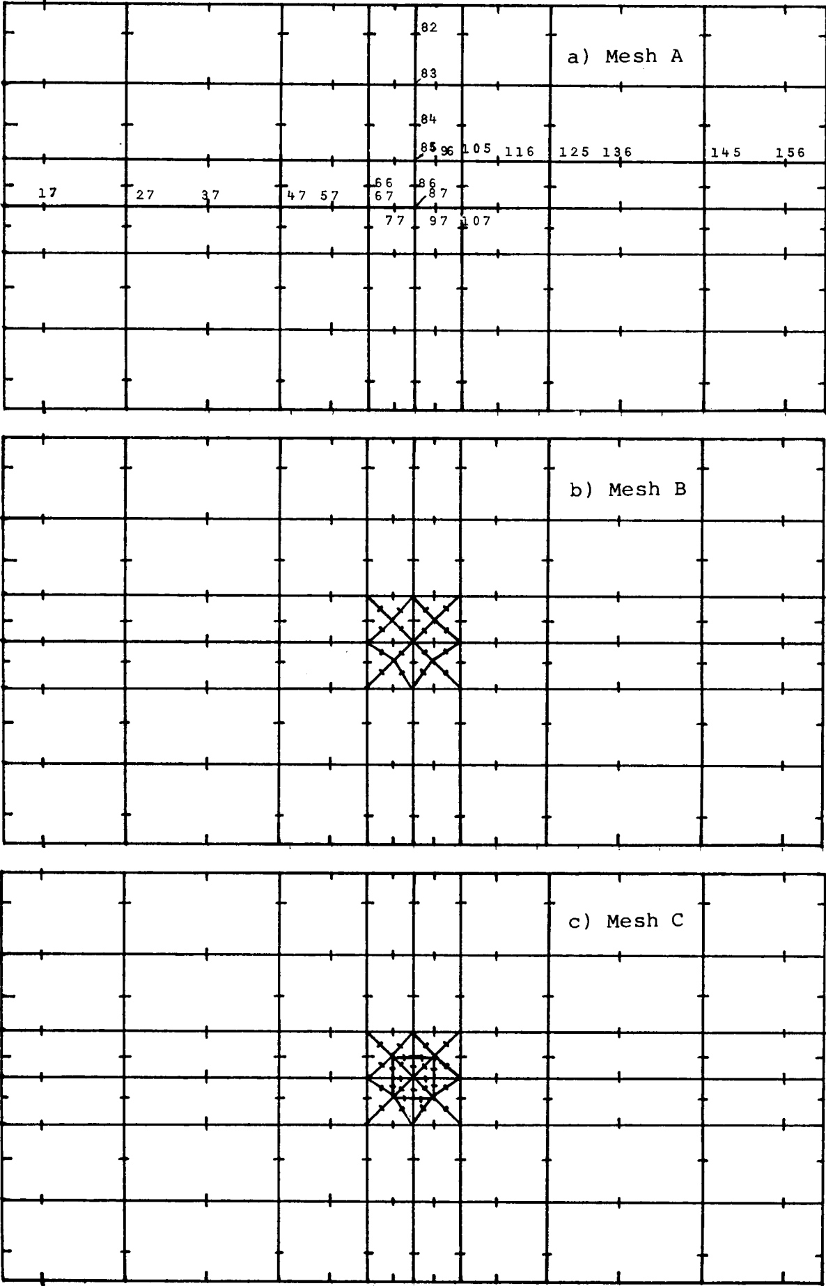
Figure 7-5 Finite Element Meshes for Two-Dimensional Verification Test
