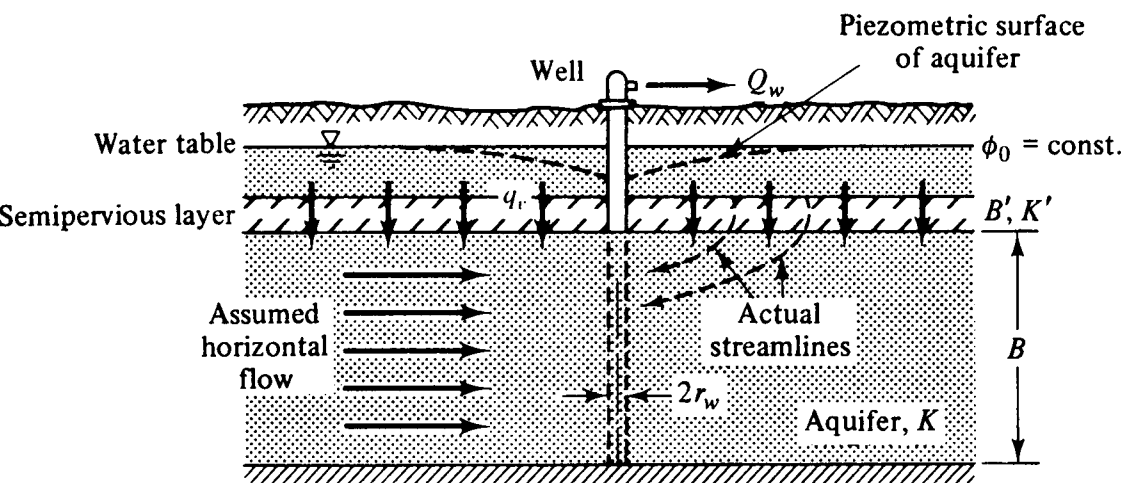
Figure 7-7: Vertical Cross-Section of Flow to a Well in a leaky, confined Aquifer (Bear, 1979)
