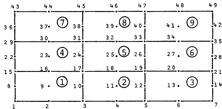
Figure 4-3 Simple 2-Dimensional Element Network
