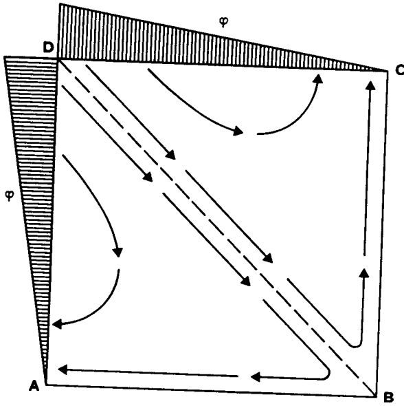
Figure 7-10: Boundary conditions for large element example
