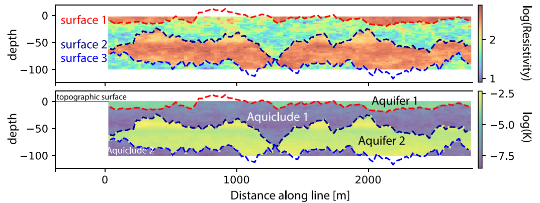
Figure 4. Cross section through one realization of a borehole-only ArchPy petrophysical model of electrical resistivity and hydraulic conductivity. In addition, the surfaces bounding the units are outlined. Note that there is a vertical exaggeration.
