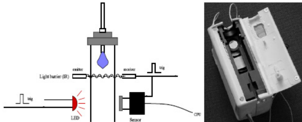
Figure 2: experimental setup and prototype
