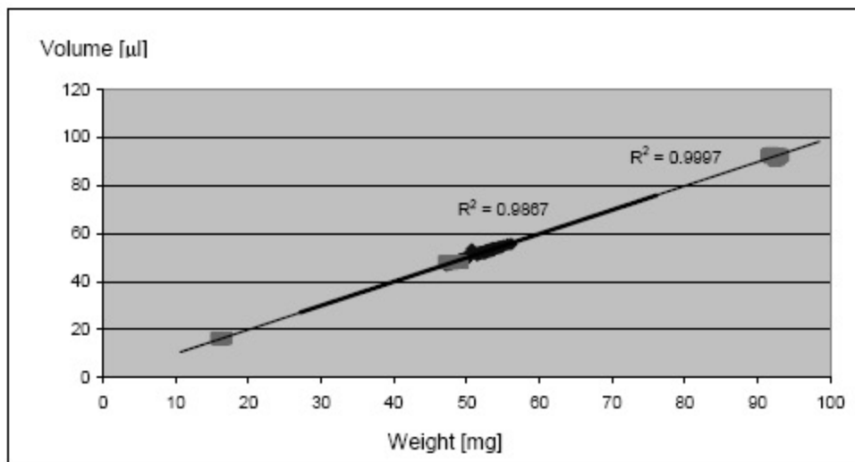
Figure 5: measurement sample results
