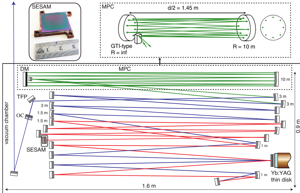
Fig. 2. Schematic of the 3.03 MHz mode-locked oscillator that delivers a pulse energy of 80 \text{ }\mu\text{J} . SESAM, semiconductor saturable absorber mirror; OC, output coupler; DM, dispersive mirror; TFP, thin-film polarizer; MPC, multipass cell; GTI, Gires-Tournois interferometer type dispersive mirror.
