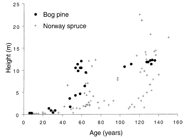
Figure 9. Scatterplot age-height for living bog pines and Norway spruces in the mixed stand of subplot LV3. In the oldest cohort, height patterns differed clearly between species, pines being of the same height, spruces showing a great height range. In contrast, trees of the second cohort showed the same pattern.
