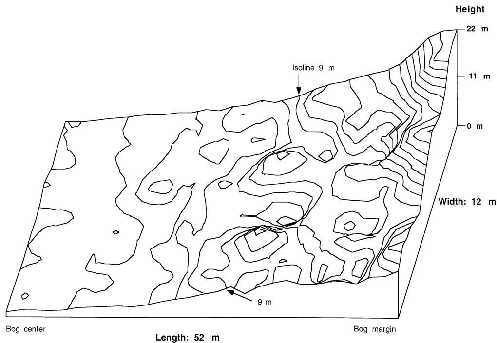
Figure 4. Three-dimensional map of the height of dominant living bog pines and Norway spruces together on the transect. Isolines of 1 metre are represented. Different scales are used for the three axes. The isoline 9 m runs approximately along the pine-spruce contact zone and along the main limit between undergrowth vegetation patches. Tree height gradient is weak in the wetter part of the transect (pine stand), but increases abruptly in the driest part (spruce stand).
