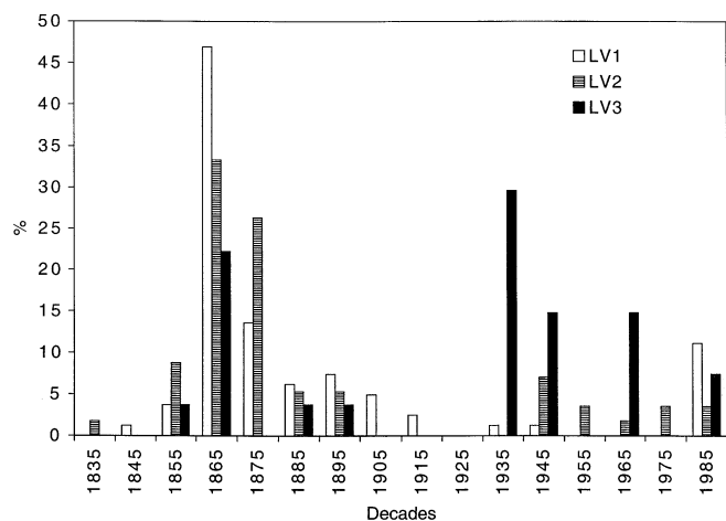
Figure 6. Living bog pine colonisation between 1830 and 1990 in the 3 subplots of the transect, given in % of the total number of individuals in each subplot.
