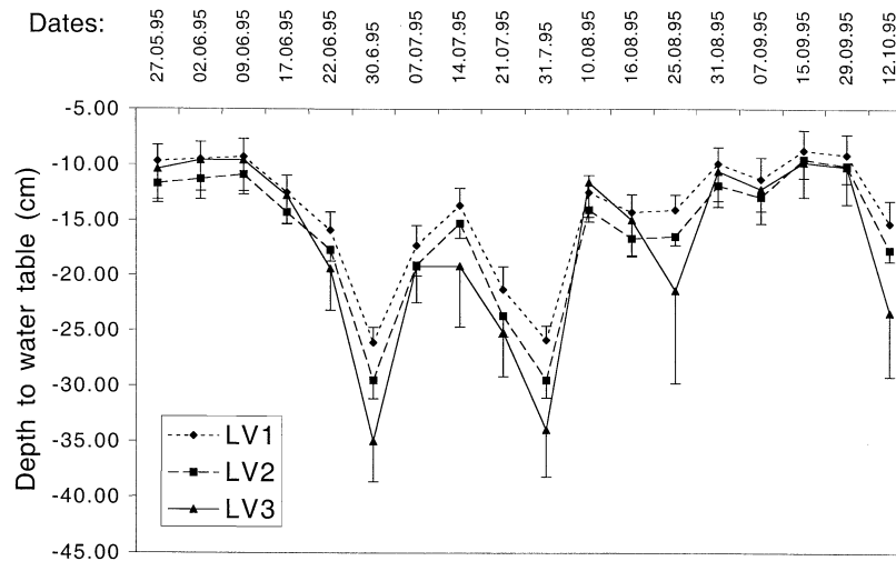
Figure 2. Measurements (mean and one SD) of depth to water table during 1995. Differences between subplots were significant with Kruskal-Wallis tests only in the driest periods: 30.6.95 ( p = 0.0055 ), 31.7.95 ( p = 0.0045 ), 25.8.95 ( p = 0.0300 ), 12.10.95 ( p = 0.0147 ).
