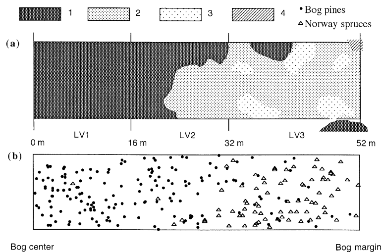
Figure 1. Main vegetation patches along the transect according to the dominant moss and herbaceous species (a) and location of the living bog pines and Norway spruces (b). 1. Wettest zone with Eriophorum vaginatum L., Sphagnum angustifolium (Russ.) C. Jens and S. fallax (Klinggr.) Klinggr.; 2. Drier zone with Vaccinium myrtillus L., Sphagnum angustifolium (Russ.) C. Jens, S. fallax (Klinggr.) Klinggr., and Polytrichum commune Hedw.; 3. Driest zone with low cover of moss and herbaceous species and with spruce litter; 4. Marginal zone with Sphagnum girgensohnii Russ. Subplots are LV1: low pine stand in the wettest zone (bog centre); LV2: intermediate pine stand; LV3: tall mixed pine and spruce stand in the driest zone (bog margin).
