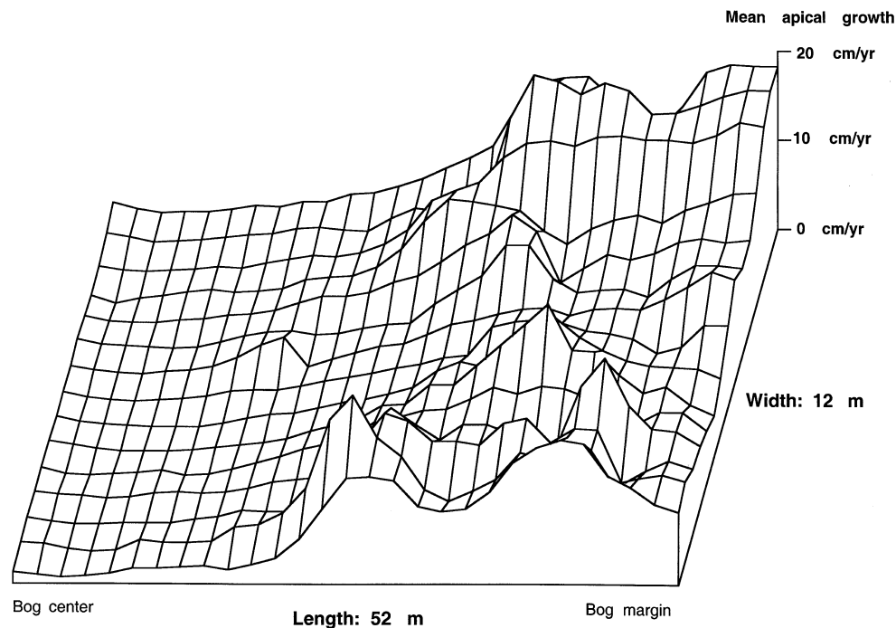
Figure 5. Three-dimensional map of mean apical annual growth of dominant living bog pines and Norway spruces together on the transect. Different scales are used for the three axes.
