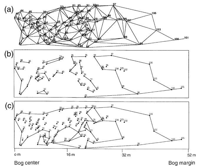
Figure 12. Clustering map according to spatial contiguity of living and dead bog pines on the transect based on the annual growth reduction values of abrupt growth change measurements of the individual trees in the period 1880–1995. Spatial constraints are given by the Delaunay's triangulation (a); maps of the fusion level at 0.85 (b) and 0.70 (c) are given. Connexity of proportional-link linkage clustering was 0.5. The main limit between groups (see c) corresponds well with the main gradients in tree species composition, tree height structure and undergrowth vegetation along the transect.
