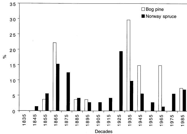
Figure 8. Living bog pine and Norway spruce colonisation between 1840 and 1990 in the mixed stand of the subplot LV3, given in % of the total number of individuals for each species. In response to the same ecological constraints, both tree species colonised the bog margin with two synchronous cohorts.
