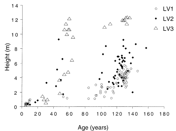
Figure 7. Scatterplot age-height for living bog pines in the three subplots of the transect. Pine colonisation occurred in two successive cohorts. Mainly for the first cohort, pine height depended on the location in the transect.
