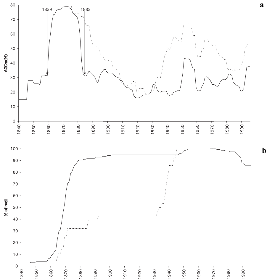
Figure 10. Abrupt growth change means (a) of bog pines on the transect and total number of radii read (b), given in %. LV1 + LV2 (continuous line) and LV3 (dotted line) are presented separately. Before 1870 AGCm curve interpretation is less reliable since it is based on few radii. Although AGCm curves showed the same trend, growth reduction was stronger (e.g. after 1880) and growth recovery weaker (e.g. before 1950) in the wettest part of the transect (LV1 + LV2) in comparison to the driest part (LV3).
