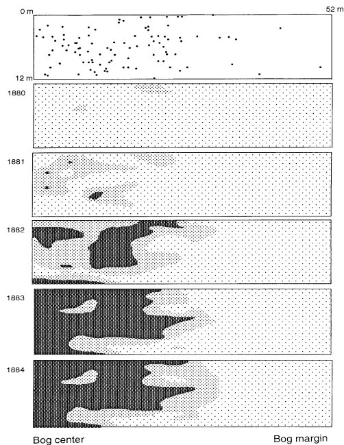
Figure 11. Two-dimensional maps of the annual radial growth reduction values given by abrupt growth change measurements of living and dead bog pine on the transect. Successive event years of the growth reduction period between 1880 and 1884 are given. The upper map represents the location of the bog pines. Dense shaded: < 30% of maximum growth; intermediate shaded: between 30 and 50% of maximum growth; light shaded: > 50% of maximum growth. AGCm growth reduction for pines was stronger in the wettest part of the transect.
