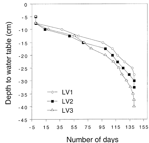
Figure 3. Duration curves of the ground-water table in the three subplots of the transect showing the cumulative number of days on which the ground water is above a certain level.
