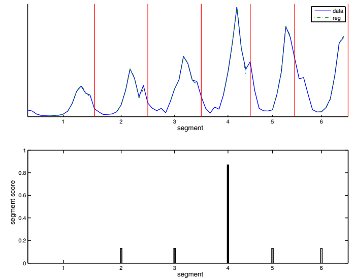
Fig. 7. Evening burglaries time series from the CICOP data set. (Top) Segmentation of the time series, with 6 change points detected. (Bottom) Output of the FIS for each segment, representing the relevance of the query (i.e., changes in trend).
