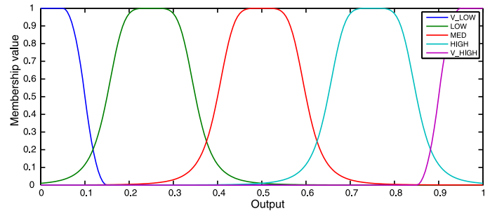
Fig. 15. Output membership functions for the FIS of the CICOP and SWX data set.
