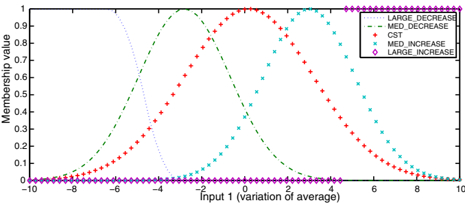
Fig. 9. Input membership functions of both evening burglaries and ATM burglaries time series.
