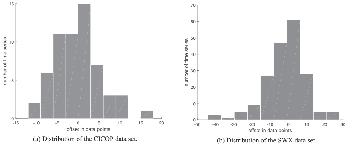
Fig. 17. Distribution (histogram) of the offsets of the 3 most significant segments of the CICOP and the SWX data sets. A negative offset indicates that the FCPD algorithm detected the point before the BFAST algorithm.
