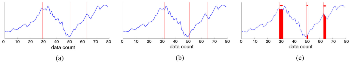
Fig. 16. Illustration of the comparison of the 3 most significant changes between the BFAST algorithm and the proposed method.
