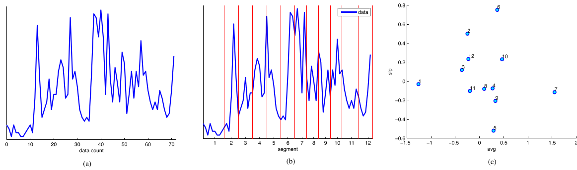
Fig. 2. Illustration of the segmentation of a time series with its shape-space representation. (a) A real time series of 72 samples. The time series has been normalized ( \mu = 0 , \sigma^2 = 1 ). From the pretty chaotic shape of the series, many change points are supposed to be found. (b) Segmentation of the time series, with K = 3 . Twelve different segments are found (represented by vertical lines). The segmentation here is based on the number of sign changes of the slope and the deviation of the predicted value. (c) Segments depicted with their shape space representation (only the first two coefficients are shown). The segments 1 and 7 are easily identified as with the lowest and highest average ( \alpha_0 ) and the segments 5 and 6 with the lowest and highest slope ( \alpha_1 ).
