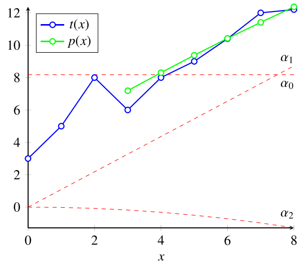
Fig. 1. A time series t(x) and its polynomial approximation p(x) with K=2 , and their coefficients. The coefficients \alpha_0 = 8.18 (estimator for the average), \alpha_1 = 1.09 (estimator for the slope), and \alpha_2 = -0.02 (estimator for the curvature) are depicted with the first term only of their respective polynomials. It should be noticed that the approximation can only start from K+1 data points.
