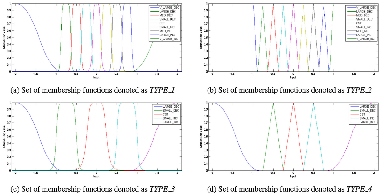
Fig. 19. Input membership functions used for the sensitivity analysis.
