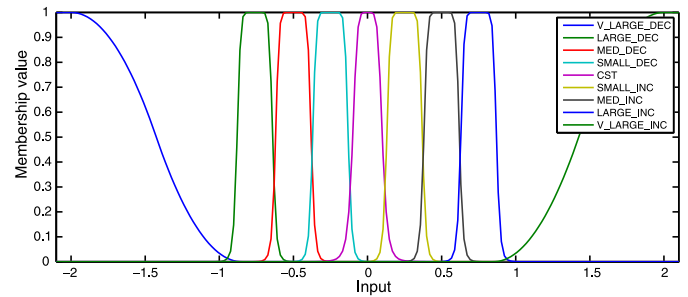
Fig. 14. Input membership functions for the FIS of the CICOP and SWX data set.
