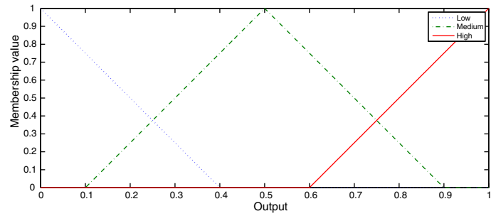
Fig. 6. Output membership functions of the cycle time series.
