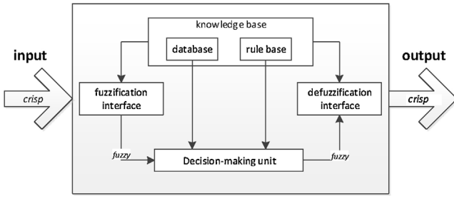
Fig. 3. Structure of a fuzzy inference system.
