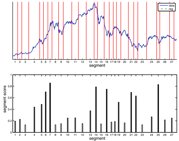
Fig. 10. The TOPIX time series. (Top) Segmentation of the time series, with 27 change points detected. (Bottom) Output of the FIS for each segment, representing the relevance of the query (i.e., finding the steepest slopes).
