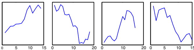
Fig. 13. Primitive shapes of the TOPIX time series, resulting from the clusters.
