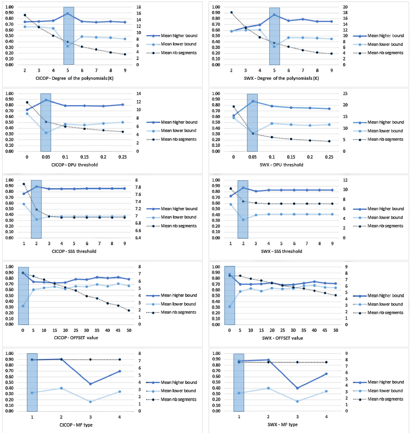
Fig. 18. (From top to bottom) Effects of a change in the parameter K , th_{DPU} , th_{SSS} , on the introduction of an offset ( OFFSET ); and on the input membership functions of the query ( MF\_TYPE ). The effects are measured on the mean lower bound and the mean upper bound of the CICOP data set (left-hand) and the SWX data set (right-hand). Lower bounds and upper bounds are calculated as the average of the 3 worst/best scores. Score values are the mean of all time series of the data set. The blue regions ( K=5 , th_{DPU}=0.05 , th_{SSS}=2 , OFFSET=0 , and MF\_TYPE=1 ) are the reference values for the comparisons.
