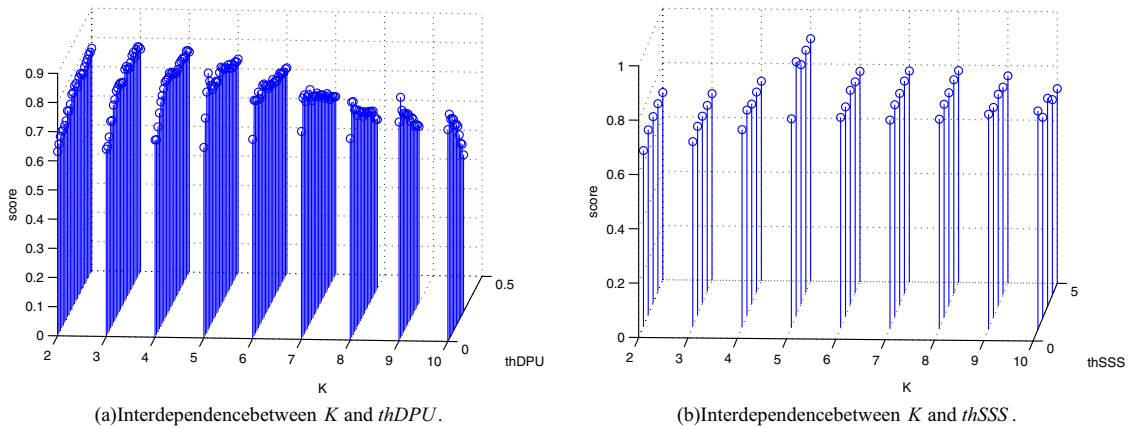
Fig. 20. Interdependence between K and the thresholds thDPU and thSSS . The scores are the mean for both the CICOP and the SWX data sets of the top 1 segment. Missing values indicate that no segmentation was found.
