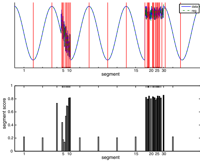
Fig. 4. The cycle time series. (Top) Segmentation of the time series, 31 change points detected. (Bottom) Output of the FIS for each segment, representing the relevance of the query.
