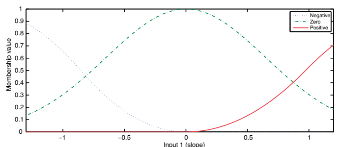
Fig. 11. Input membership functions of the TOPIX time series.
