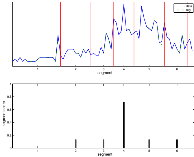
Fig. 8. ATM break-ins time series from the CICOP data set. (Top) Segmentation of the time series, with 6 change points detected. (Bottom) Output of the FIS for each segment, representing the relevance of the query (i.e., changes in trend).
