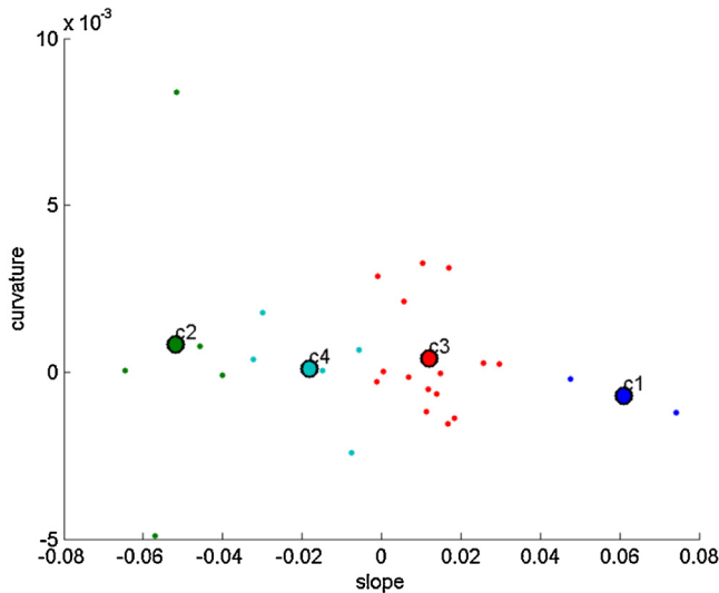
Fig. 12. Clustering of the segments from the TOPIX time series. The segments are described with their slope and their curvature.
