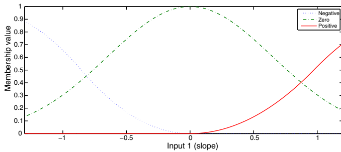
Fig. 5. Input membership functions of the cycle time series.
