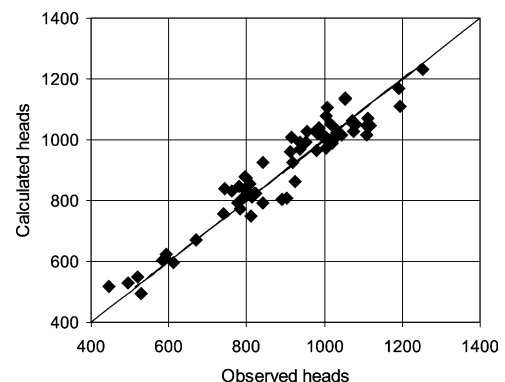
Fig. 13. Scatter diagram for observed and simulated heads in 71 boreholes, Variant 1; calculated variance is 2550 m 2 .
