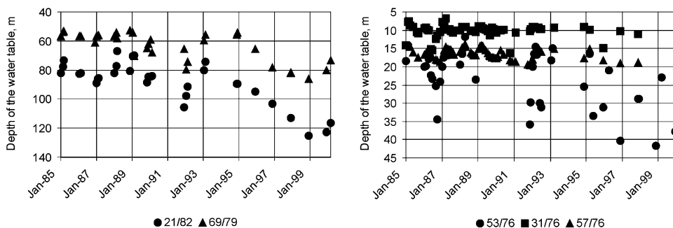
Fig. 4. Progressive increase in the depth of the ground water table in the extraction boreholes with serial numbers 53/76, 31/76, 57/76, 21/82 and 69/79 during non-pumping seasons (October to March).
