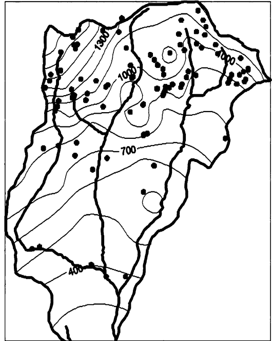
Fig. 9. Piezometric map constructed from interpolated piezometric heads for March 2000.
