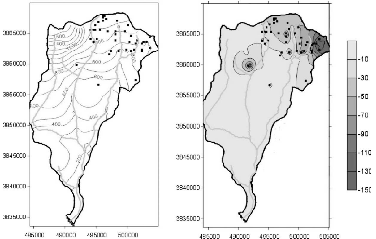
Fig. 16. Results of simulation with 8.77 Mm 3 annual groundwater pumping: Left—piezometric map; Right—differences to the basic variant (colour scale is in metres).
