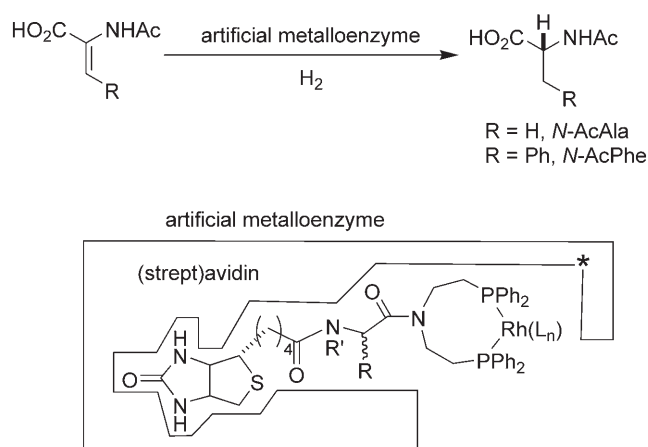
Scheme 1. Second generation artificial metalloenzymes based on the biotin-avidin technology for the reduction of N -acetamidoalkenes. The host protein [(strept)avidin] displays high affinity for the anchor (biotin); introduction of an enantiopure \alpha -amino acid spacer, combined with a flexible diphosphine ligand allows us to chemically optimize both the activity and the selectivity. Site-directed mutagenesis further enables a genetic optimization of the host protein to afford enantioselective artificial hydrogenases.
