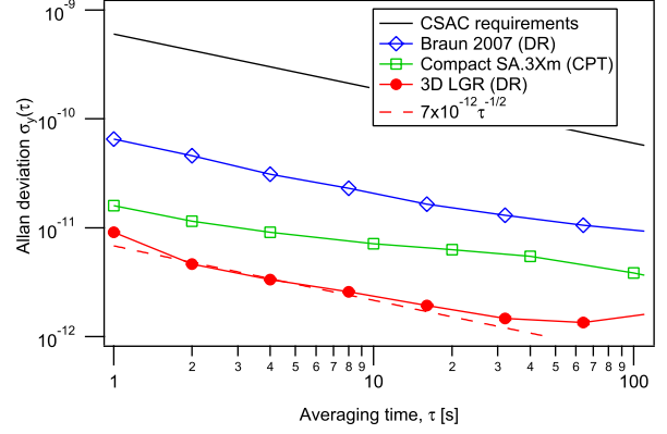
Fig. 12. Clock frequency instability measured with the \mu -LGR (filled red bullets), compared to the stabilities of a commercially available clock based on coherent population trapping (CPT, open green squares) [30], and the miniature DR-based clock of reference (open blue diamonds) [10]. The solid black line gives the performance goal for the DARPA CSAC project [9].
