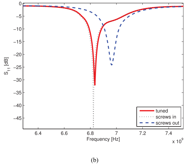
Fig. 7. (a) Comparison between the reflection coefficient of one measured prototype ( t = 2.0 mm, tuned) and model simulation for t = 2.0 mm with maximum insertion of the two screws. The resonance frequency f_r is slightly higher in the measured prototype due to fabrication and assembly tolerances. (b) Measured frequency tuning of the \mu -LGR prototype ( t = 2.0 mm) around 6.835 GHz, for different positions of the tuning screws.
