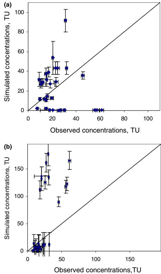
Fig. 14. Scatter diagram between observed and simulated ^3\text{H} concentrations: (a) variant with "high" input porosity; (b) variant with "low" input porosity. Bars represent uncertainty of observed and simulated values, respectively.
