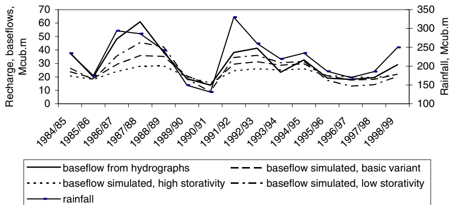
Fig. 10. Comparison of transient baseflows, separated from hydrographs, with those simulated by the numerical models with different input storativities.
