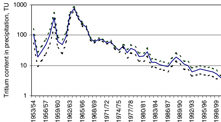
Fig. 3. Input function for ^3\text{H} content of the precipitation over the Kouris catchment. Dashed lines limit the range of the uncertainty.
