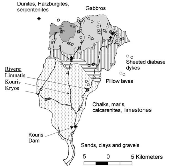
Fig. 2. Geological map of the Kouris catchment with sampling locations: crosses – precipitation; circles – boreholes; triangles – springs; squares – rivers.
