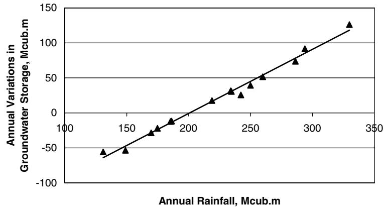
Fig. 6. Regression between annual rainfall and variations in groundwater storage for the entire Kouris catchment for the years 1984–1999.
