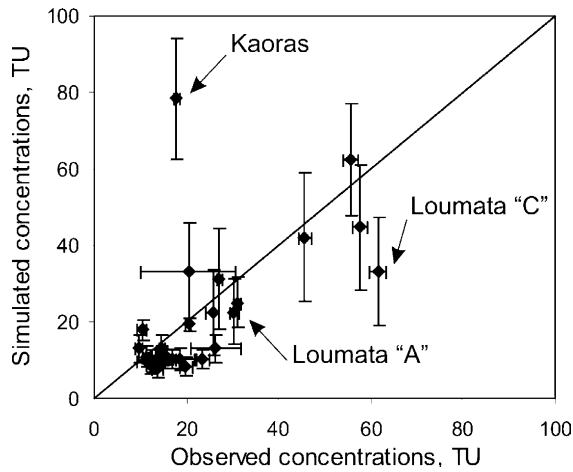
Fig. 12. Scatter diagram between observed and simulated ^3\text{H} concentrations (best fit) with the uncertainty ranges.
