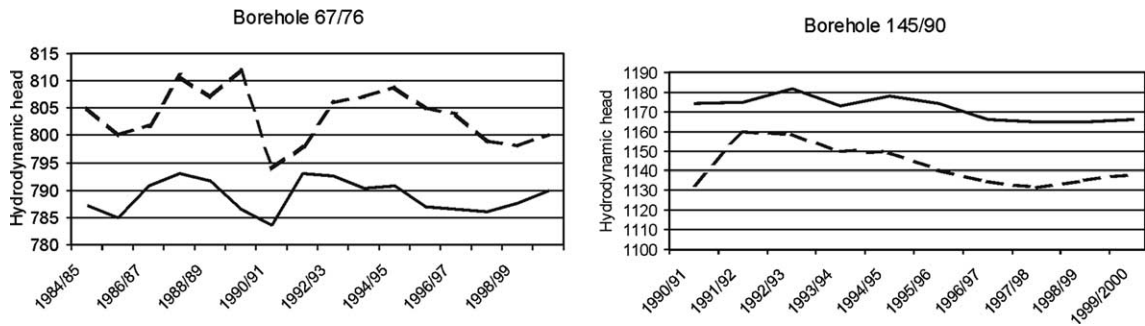
Fig. 9. Examples of comparison between observed (solid lines) and simulated (dashed lines) transient piezometric heads for the boreholes 67/76 and 145/90.
