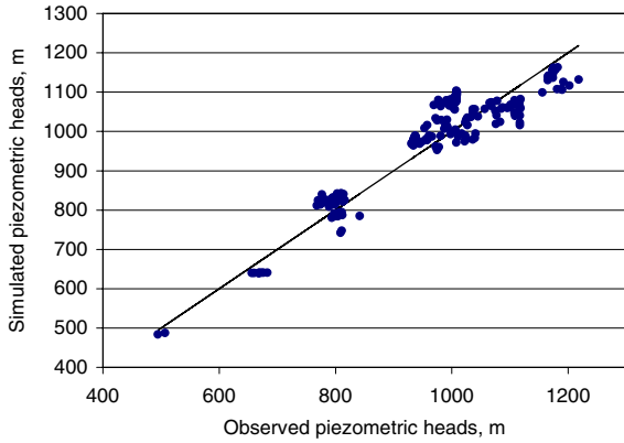
Fig. 8. Scatter diagram of 210 observed and simulated transient piezometric heads for the basic variant.
