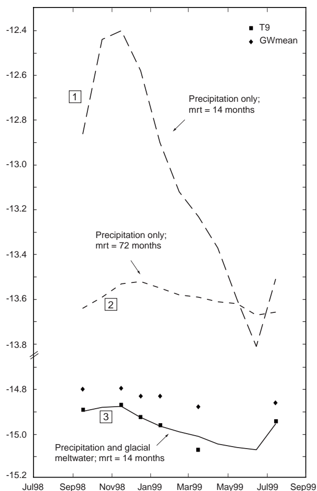
Figure 8. Observed \delta^{18}\text{O} data at station T9 and calculated mean signal of remaining ground water sampling stations (GWmean). Indicated is the output function for lumped-parameter modeling representing the best fit to the observed data when the precipitation-derived input function is modified by an additional meltwater component (line 3). Line 1 illustrates the output function for solely precipitation-derived input function for identical model parameters of the best fit model. Even for potential large residence times (line 2), the output function from the precipitation-derived input function remains enriched compared to the observed data (mrt = mean residence time).
