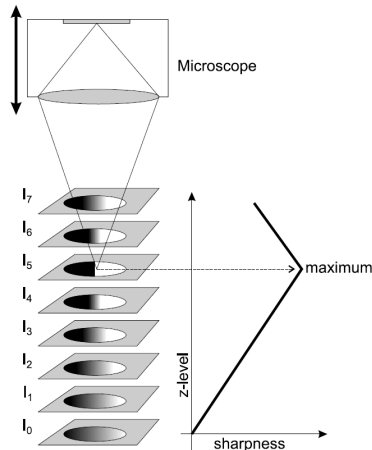
Figure 2. Multifocus 3D microscopy: measurement principle
