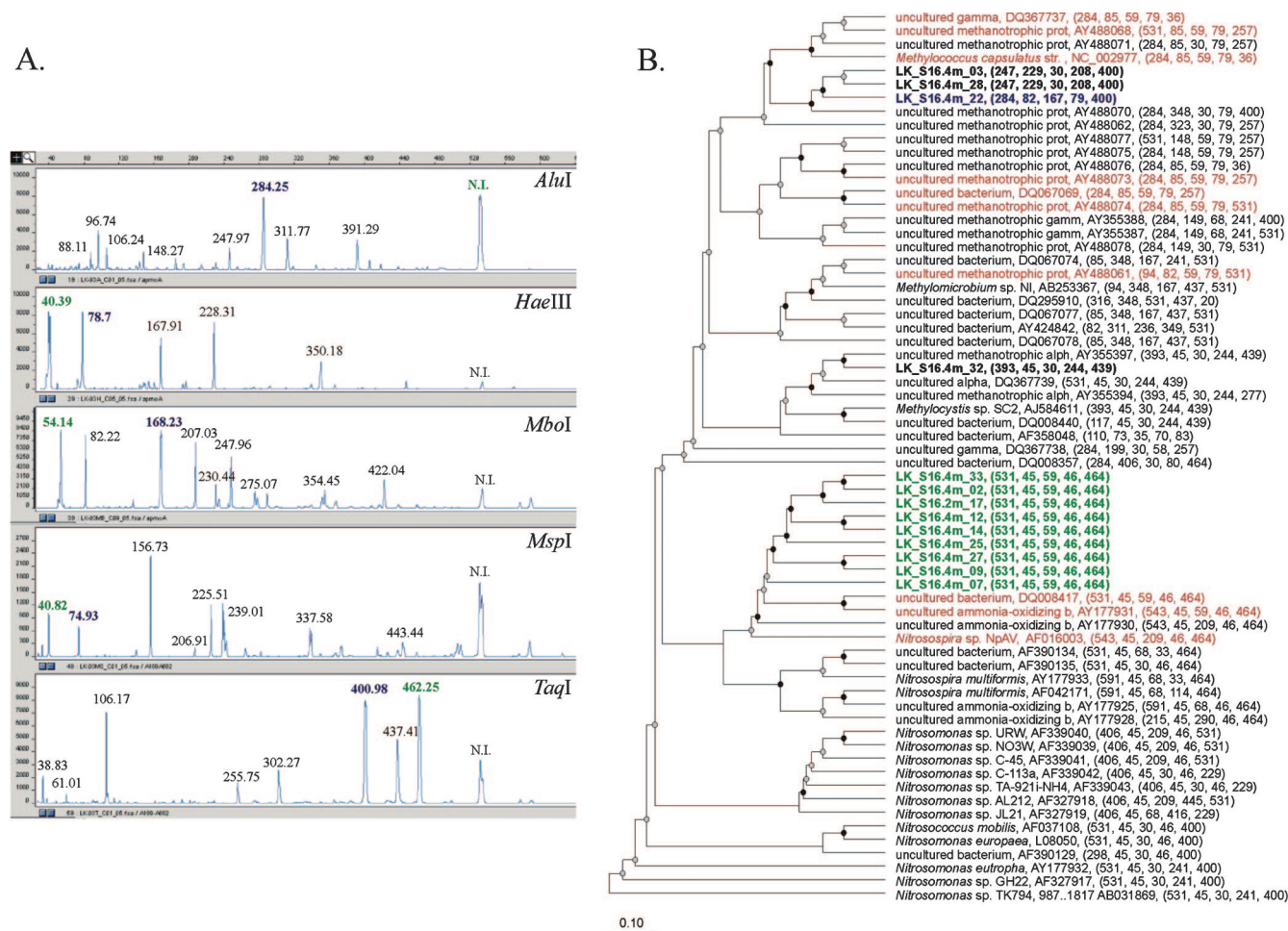
FIG. 2. Validation of the identification function of TRiFLE using experimental results from a T-RFLP experiment using a water sample at the metalimnetic layer of Lake Kinneret (Israel). (A) Electropherograms of the T-RFLP analysis of pmoA and amoA PCR products digested with HaeIII, MspI, MboI, AluI, and TaqI. T-RFs from a control set of clones that were identified by the program are shown in blue and green (colors indicate different phylogenetic groups). "N.I." indicates undigested peaks that were omitted for the calculation of the distance. (B) Phylogenetic tree of the reference data set of sequences used for the identification, including 13 clones from a library prepared from the environmental sample (bold). The simulated T-RF lengths calculated with TRiFLE for each of the enzymes are given in parentheses. The phylogenetic analysis was carried out using ARB ( http://magnum.mpi-bremen.de/molecol/arb/ ); bootstraps values are indicated by black (100%) or gray (90 to 99%). The top 20 sequences identified by the program (see Table 2) are shown in color. Sequences in blue and green correspond to clones from the control set. Sequences in red correspond to reference sequences among the top 20. b, bacterium; prot, proteobacterium; alpha or alpha, alphaproteobacterium; gamma or gamma, gammaproteobacterium; str., strain.
