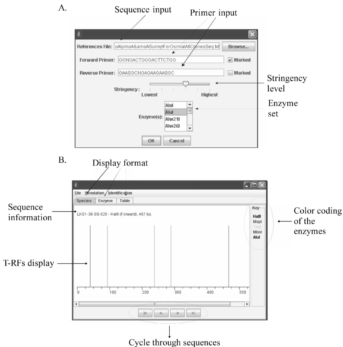
FIG. 1. Input interface of TRiFLe for simulating T-RFs (A) and graphical display of the results from the simulation (B). The different parts of the displays are indicated.
