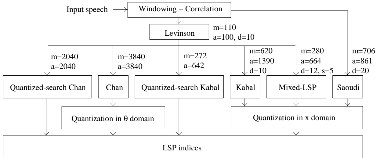
Figure 3: Computational complexity of different LSP calculation methods (10 th -order LPC system) (M=multiplications, A=add/sub, D=divisions, S=square roots).
