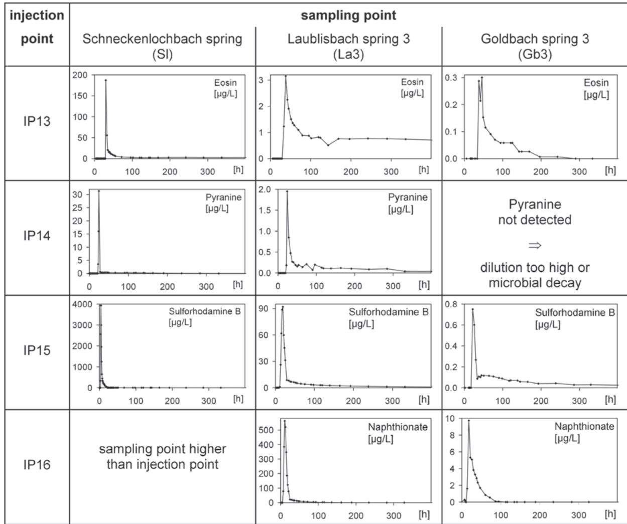
Fig. 9. Selected breakthrough curves from the western Hochifen-Gottesacker area. The curves in La1 , 2 and 4 are similar to those in La3 and are not presented here; minor traces of Sulforhodamine were detected at Si ; no positive results were obtained for Rb , Gb1 , 2 and 4.
