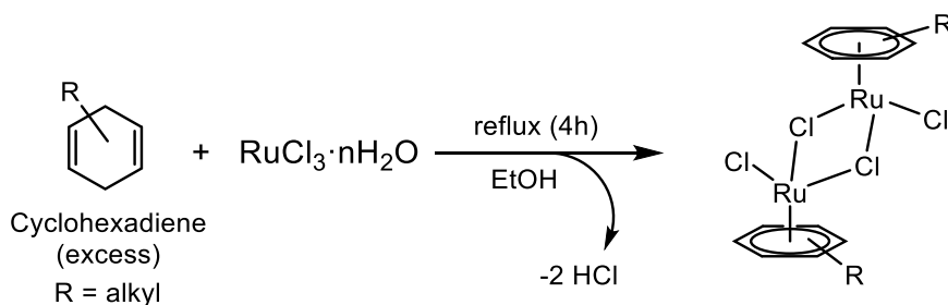
Scheme 2. Synthesis of arene ruthenium dimers.
