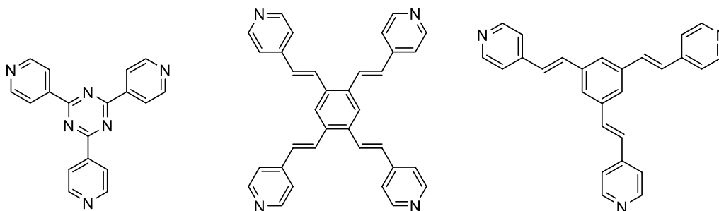
Figure 12. Panel ligands used to give rise to prismatic or cubic metallacages. From left to right: 2,4,6-tri(pyridin-4-yl)-1,3,5-triazine, 1,2,4,5-tetrakis{2-(pyridin-4-yl)vinyl}benzene and 1,3,5-tris{2-(pyridin-4-yl)vinyl}benzene.
