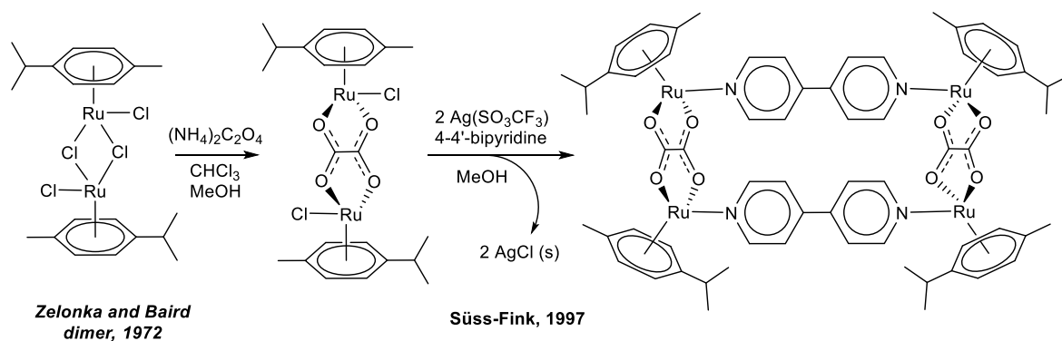
Scheme 1. Synthesis in 1997 of a metalla-rectangle by Süss-Fink and co-workers.
