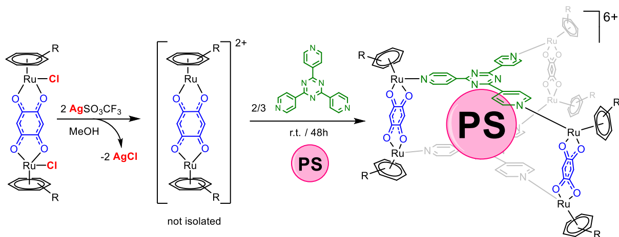
Scheme 5. Synthesis of the metallacages with PS in the inner cavity.
