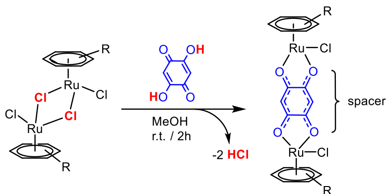
Scheme 3. Synthesis of arene ruthenium clips.
