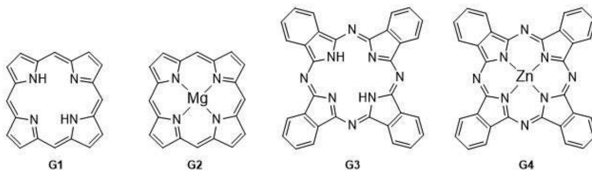
Figure 14. Photosensitizers used in this work. From left to right: 21 H ,23 H -porphine ( G1 ), Mg(II)-porphine ( G2 ), 29 H ,31 H -phthalocyanine ( G3 ) and Zn(II)-phthalocyanine ( G4 ).
