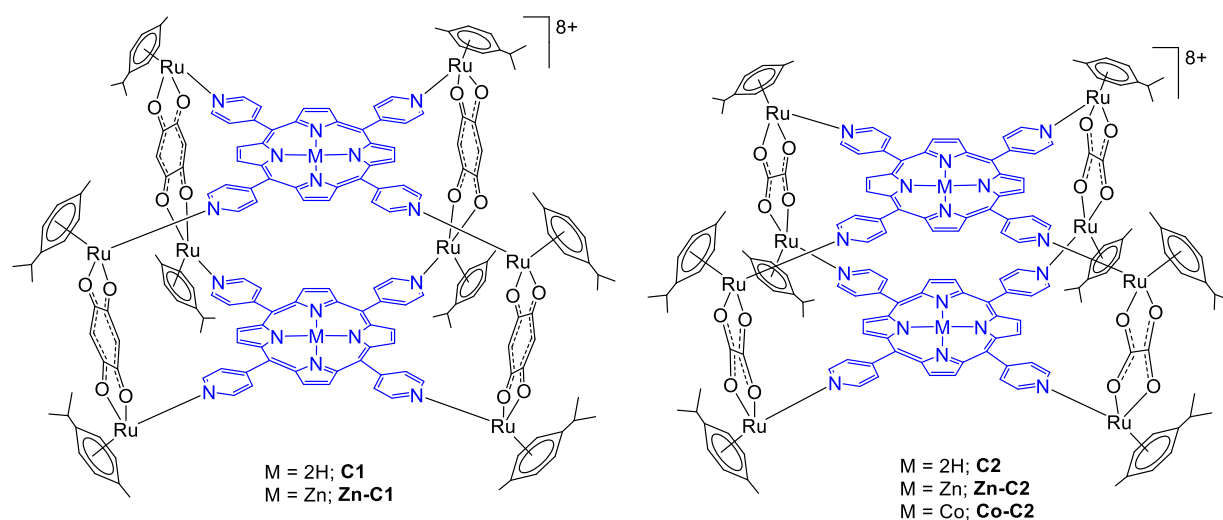
Figure 20. Arene ruthenium metallacages used in this work. All octa-cationic assemblies were isolated as their triflate salts. In blue is showed the tetrapyrrolylporphyrins, forming part of the metallacage structure as the ligand panels.
