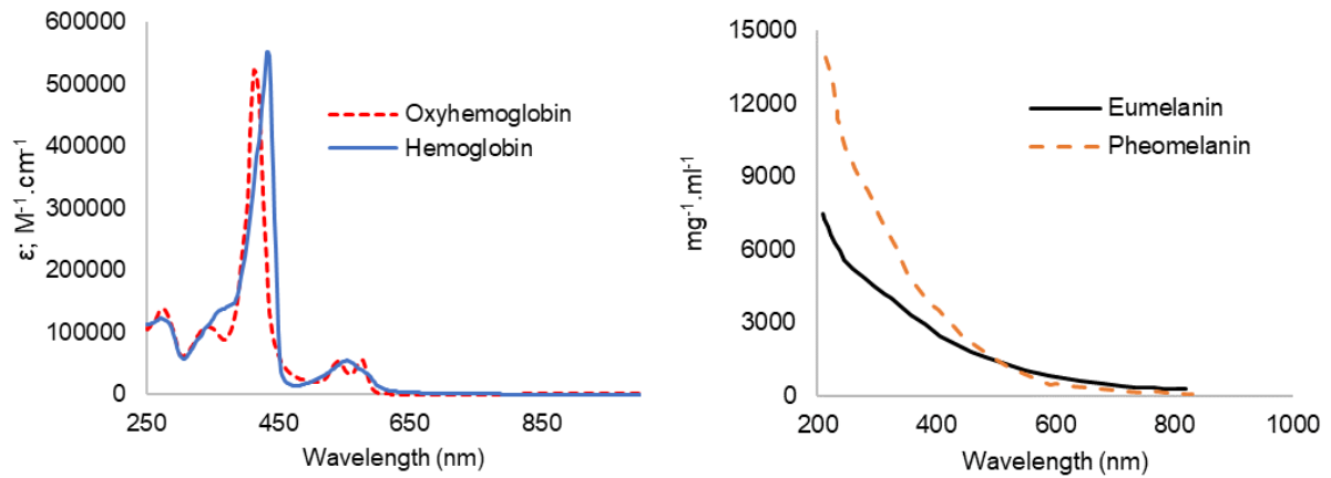
Figure 4. Left; absorption of oxyhemoglobin (red) and hemoglobin (blue) in the visible spectrum. The molar extinction coefficients were compiled by Scott Prahl using data from W. B. Gratzner, Med. Res. Council Labs, Holly Hill, London and N. Kollias, Wellman Laboratories, Harvard Medical School, Boston. Right; absorption of Eumelanin (black) and Pheomelanin (orange), two types of melanin in human [15].
