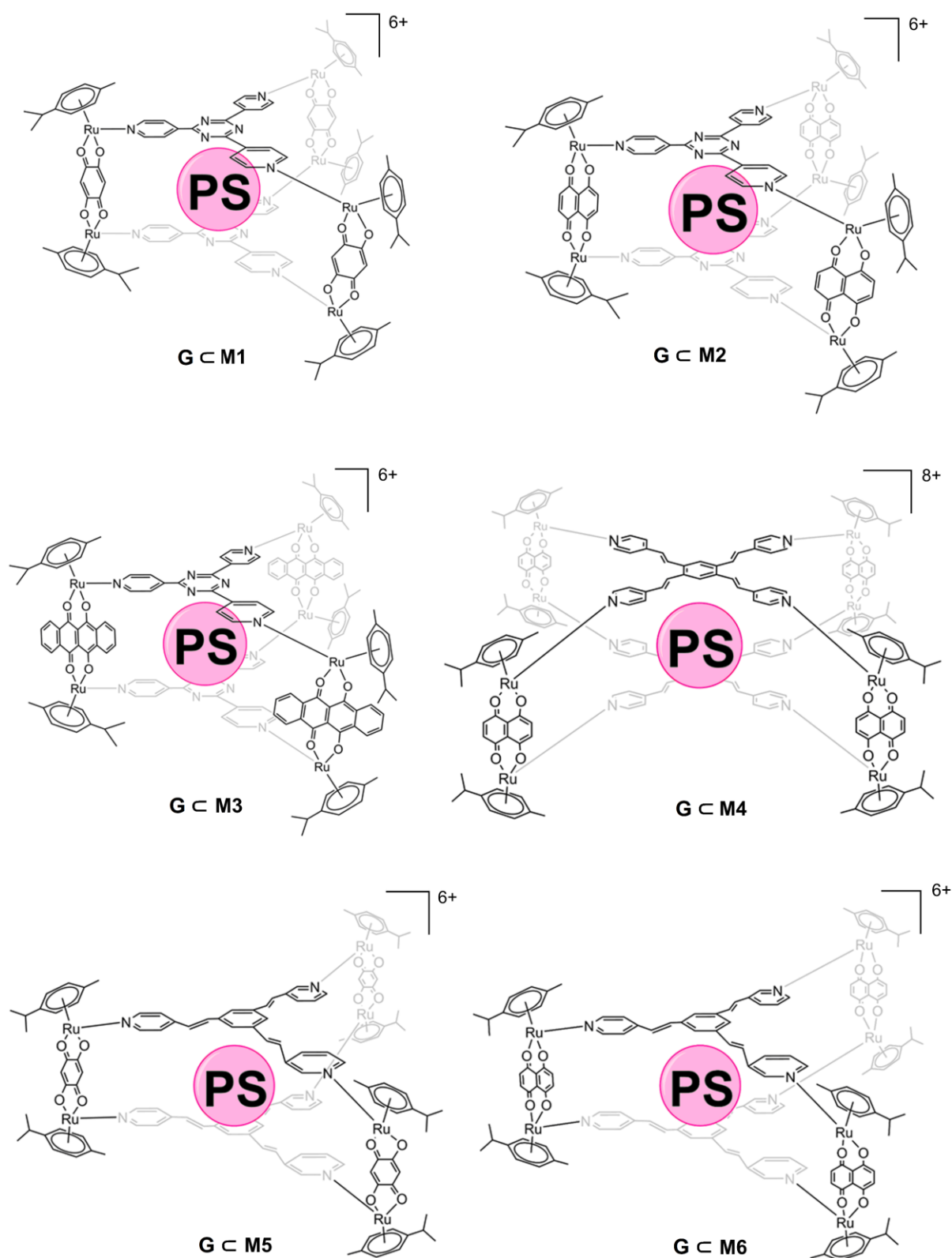
Figure 15. Structures of ruthenium(II) metallacages used in this work. The photosensitizer (G) is represented by a sphere (PS). 21H,23H-porphine (G1) was hosted in M1–M6 , Mg(II)-porphine (G2) in M1 , M4 , and M6 , 29H,31H-phthalocyanine (G3) and Zn(II)-phthalocyanine (G4) in M4–M6 .
