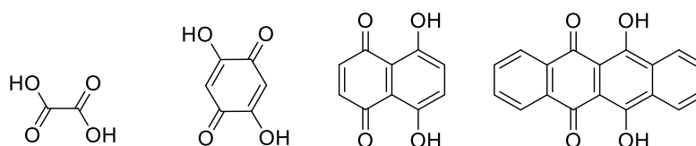
Figure 11. Protic ligands used as spacer in the arene ruthenium bimetallic complex. From left to right: oxalic acid, 2,5-dihydroxy-1,4-benzoquinone, 5,8-dihydroxy-1,4-naphthoquinone and 6,11-dihydroxy-5,12-naphthacenedione.
