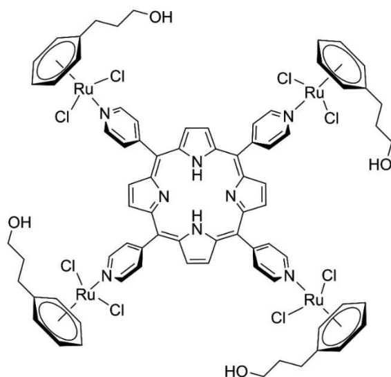
Figure 26. Structure of functionalized tetrapyridylporphyrin arene ruthenium complex.
