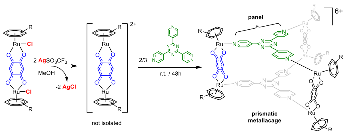
Scheme 4. Synthesis of metallacages.
