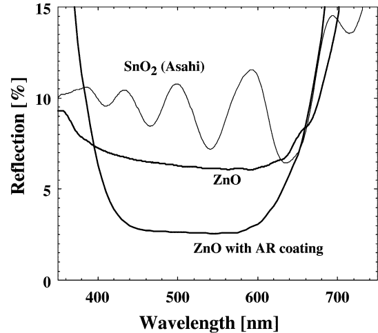
Fig. 1. Comparison of the reflection behaviour (from the glass side) of amorphous p-i-n cells deposited on \text{SnO}_2 (Asahi U), on LP-CVD ZnO and on LP-CVD ZnO with an AR-coating. The AR reduces the reflectance by approximately 4%.
