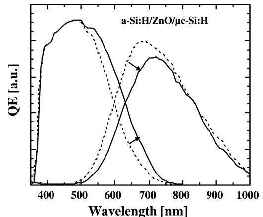
Fig. 6. Impact of the intermediate TCO layer on the QE of the a-Si:H top and \mu\text{c-Si:H} bottom cells. The dashed lines show the tandem without the interlayer, the solid lines represent the one with the incorporated intermediate TCO layer.
