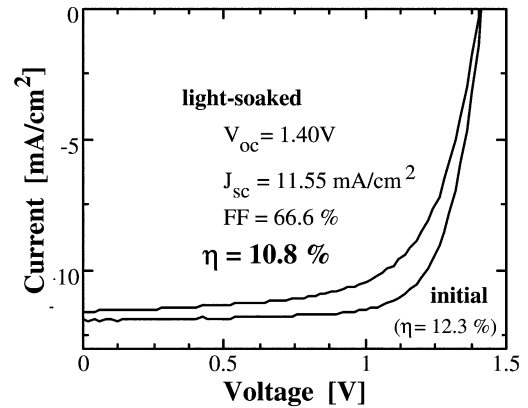
Fig. 5. AM1.5 I - V characteristics of a micromorph tandem test cell deposited on glass/LP-CVD ZnO in the initial state and after 1000 h of light-exposure (1 sun at 50 °C). The \mu\text{c-Si:H} bottom cell has a thickness of 2 \mu\text{m} .
